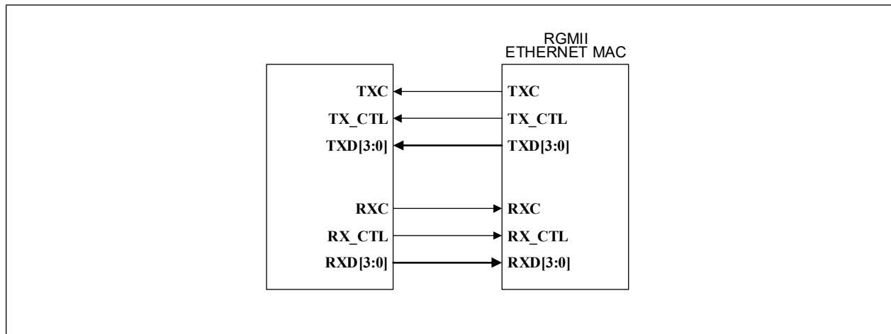
FIGURE 5-18: RGMII INTERFACE
