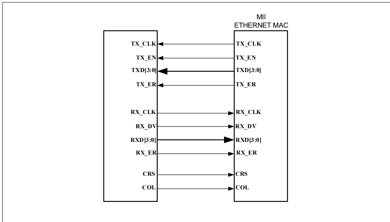
FIGURE 5-17: MII INTERFACE
