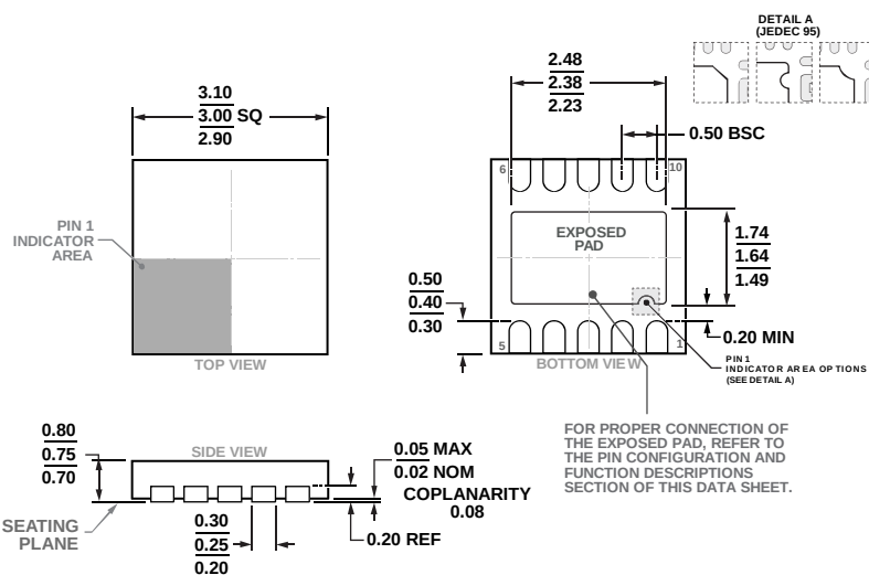
Figure 70. 10-Lead Lead Frame Chip Scale Package [LFCSP] 3 mm × 3 mm Body and 0.75 mm Package Height (CP-10-9)
