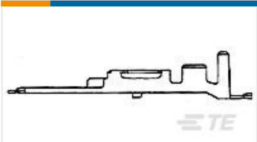
TE Part #172777-1 MIC MARE-2 TAB CONTACT
