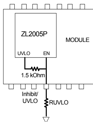
Figure 12. UVLO Circuit
