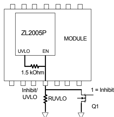
Figure 13. INHIBIT Circuit
