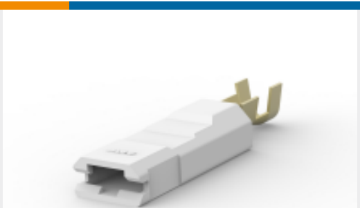
TE Part #520988-1 ULTRA POD: Straight, Receptacle Assembly, Unplated, .250 inch
