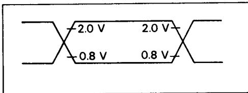
Figure 17. Reference Level (Input)
