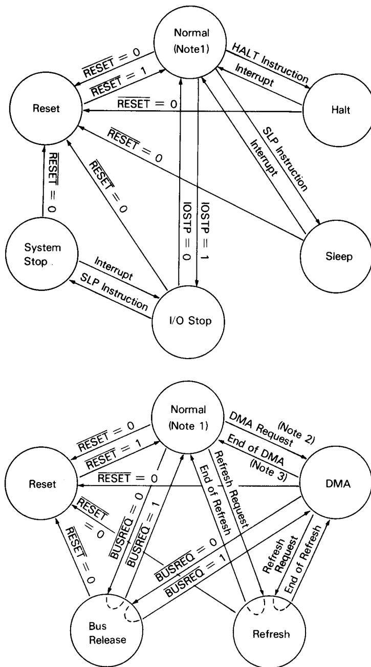
Figure 19. Operation Mode Transitions
