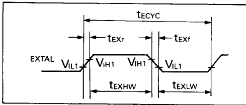
Figure 14. External Clock Rise Time and Fall Time
