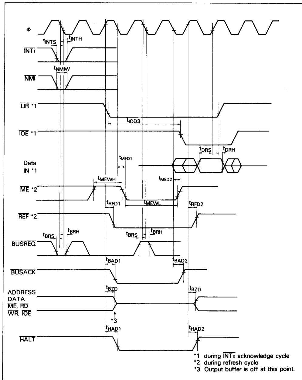
Figure 5. CPU Timing ( INT_0 Acknowledge Cycle, Refresh Cycle, Bus Release Mode, Halt Mode, Sleep Mode, System Stop Mode When \overline{IOC} = 1 )
