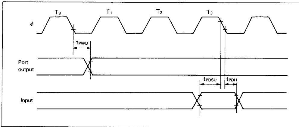
Figure 13. Port Input and Output Timing
