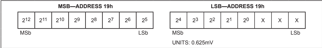
Figure 50. AverageV CELL Register Format (Output)
