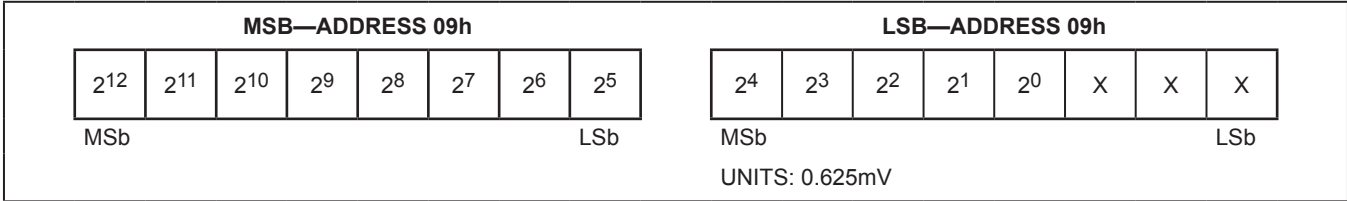
Figure 49. V CELL Register Format (Output)
