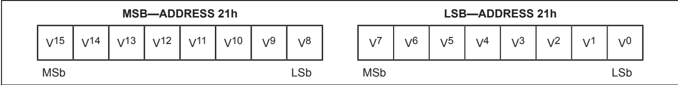
Figure 48. Version Register Format (Output)
