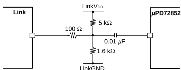
(b) Link-on Isolation Barrier Circuit
