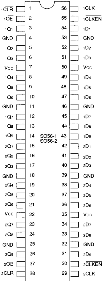
SSOP TSSOP TOP VIEW
