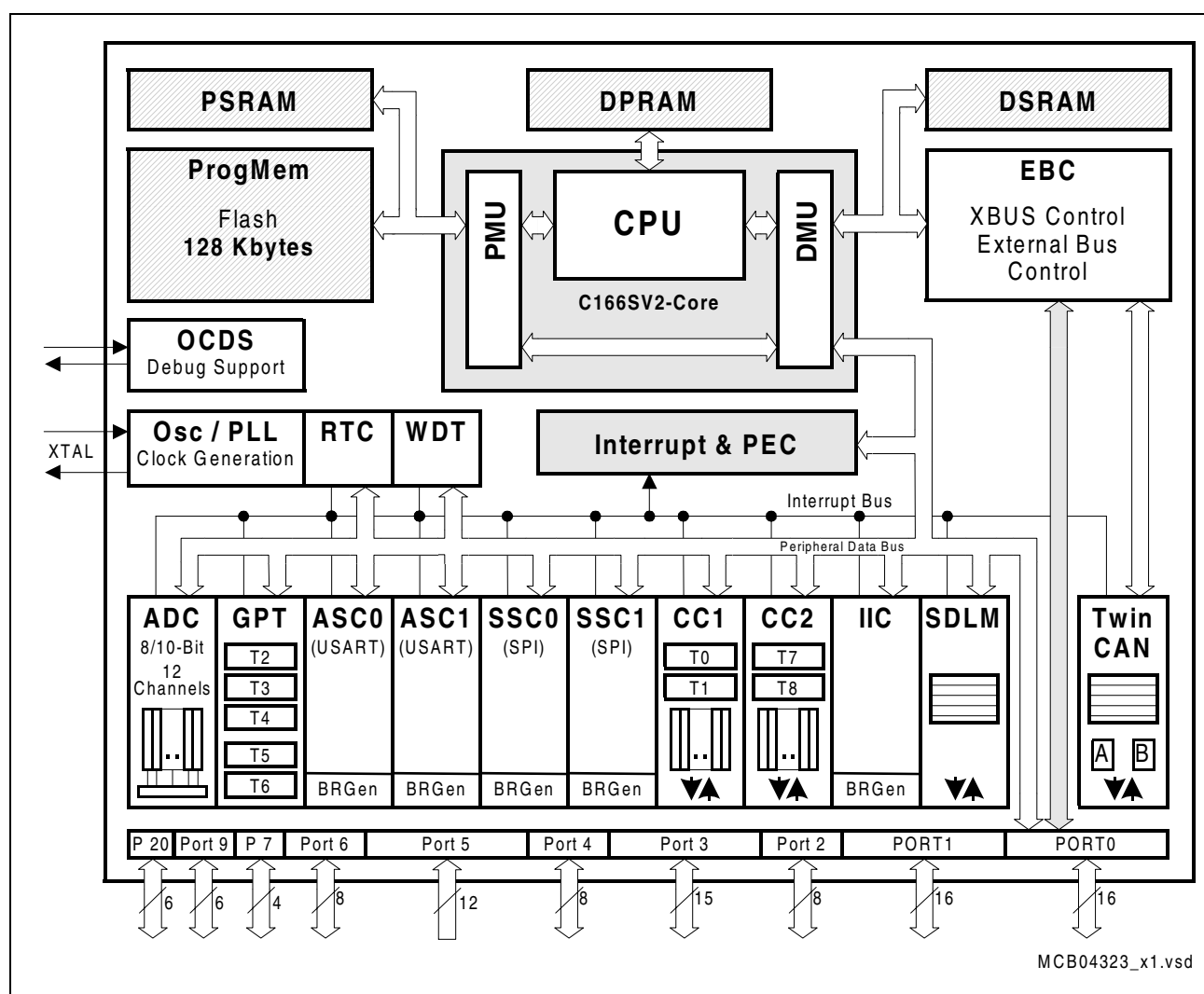
Figure 3 Block Diagram
