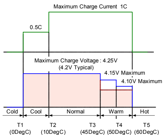
Figure 7: NTC Window
