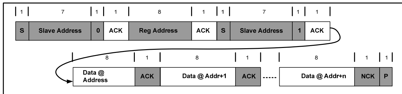
Figure 23: Multi-Read
