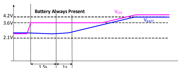
b) Charging Start-Up with Battery Present
