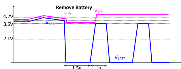
c) Remove Battery during Charging
