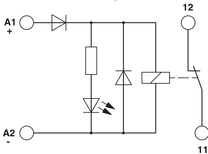
Circuit diagram
