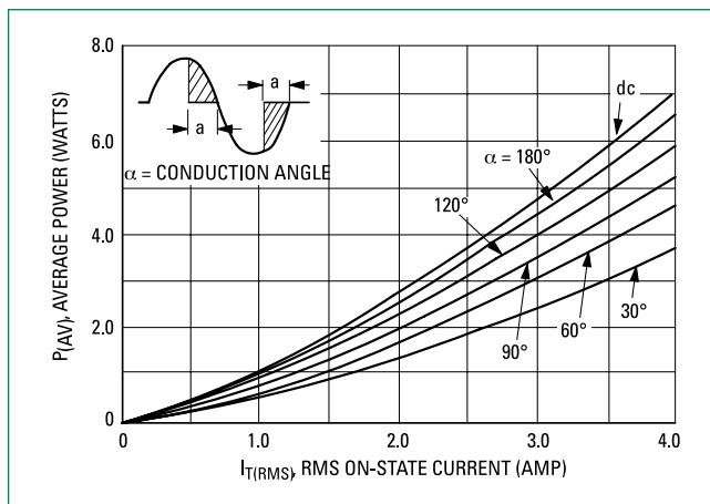
Figure 4. Power Dissipation
