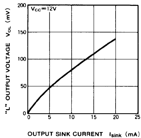
"L" OUTPUT VOLTAGE VS. OUTPUT SINK CURRENT
