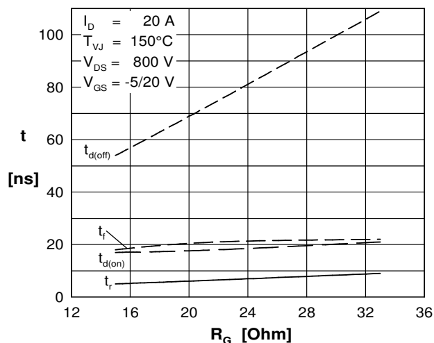
Fig. 16 Typical switching time versus external gate resistor
