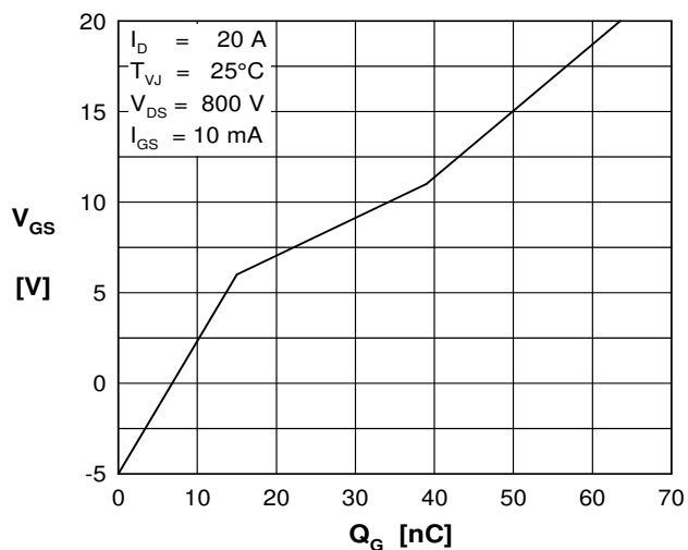
Fig. 17 Typical turn on gate charge, trendline
