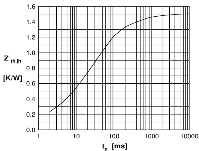
Fig. 18 Typical transient thermal impedance
