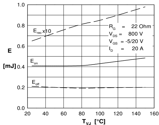
Fig. 14 Typical switching energy versus temperature
