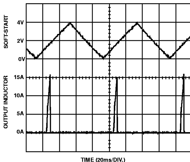
FIGURE 4. OVER-CURRENT OPERATION
