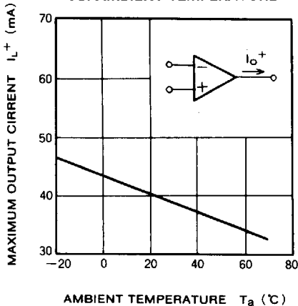
MAXIMUM OUTPUT CURRENT VS. AMBIENT TEMPERATURE
