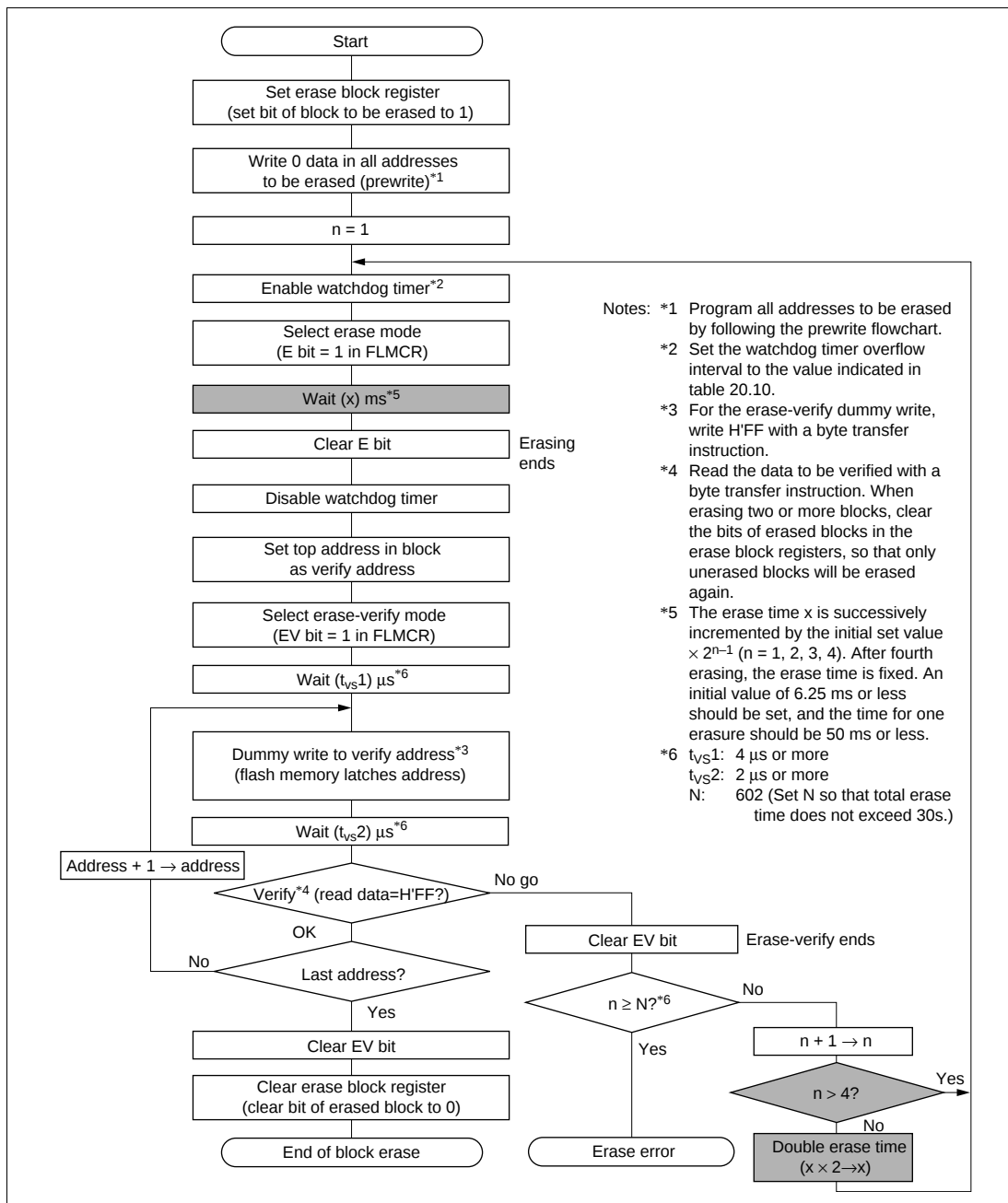
Figure 20.9 Erasing Flowchart
