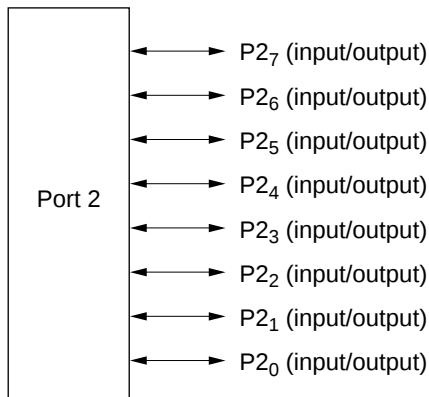
Figure 7.8 Pin Functions in Mode 3 (Port 2)
