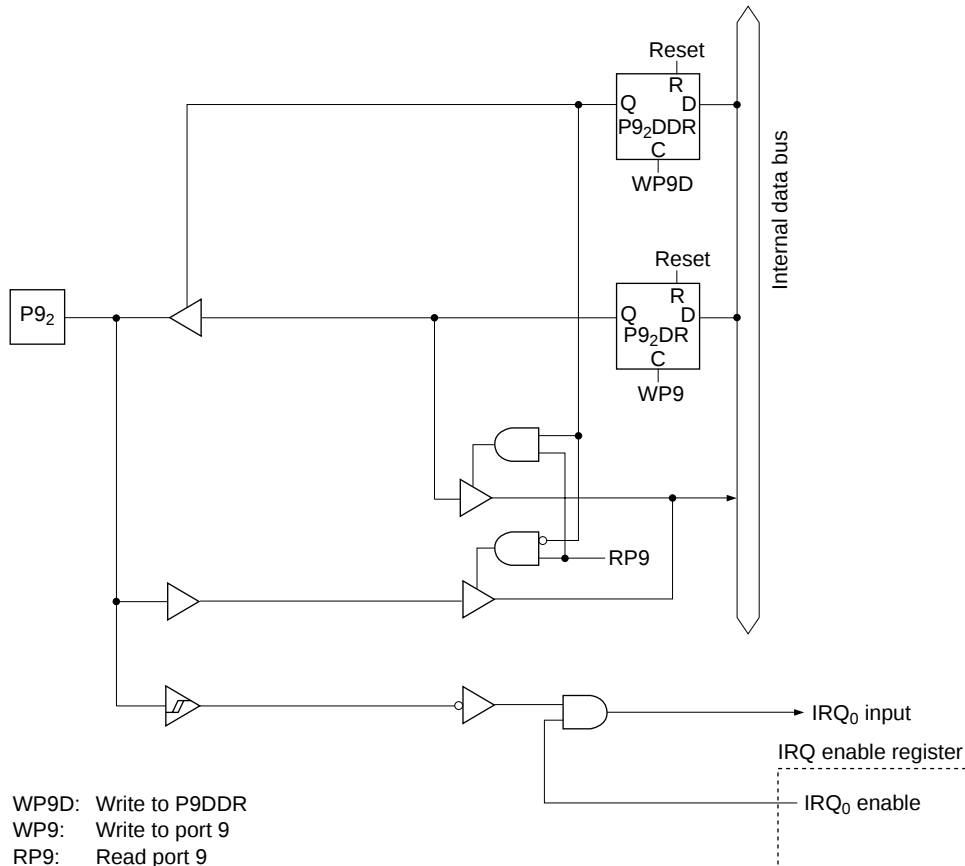
Figure C.9 (c) Port 9 Block Diagram (Pin P9 2 )
