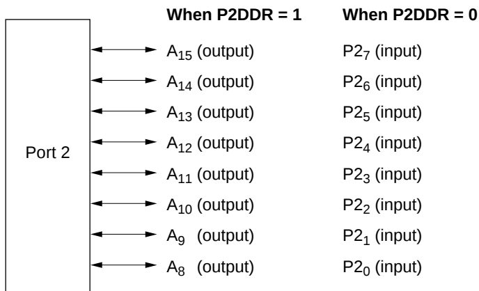
Figure 7.7 Pin Functions in Mode 2 (Port 2)
