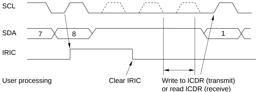
Figure 13.10 IRIC Set Timing and SCL Control
