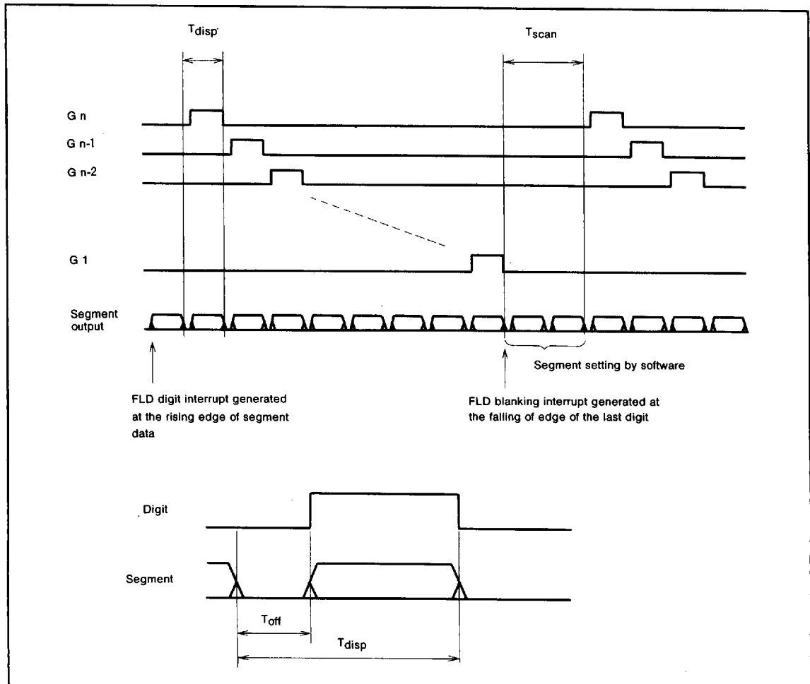
Fig. 33 FLDC timing
