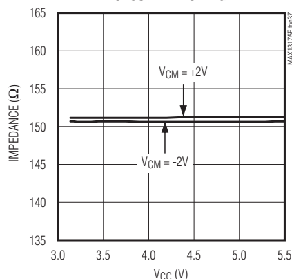
V.35 COMMON-MODE IMPEDANCE vs. SUPPLY VOLTAGE
