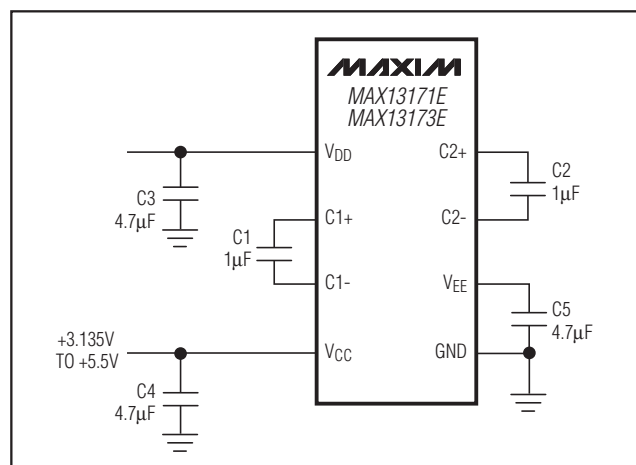
Figure 15. Charge Pump
