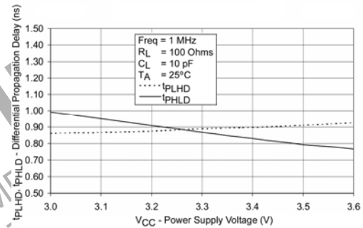
Figure 13. Differential Propagation Delay vs. Power Supply
