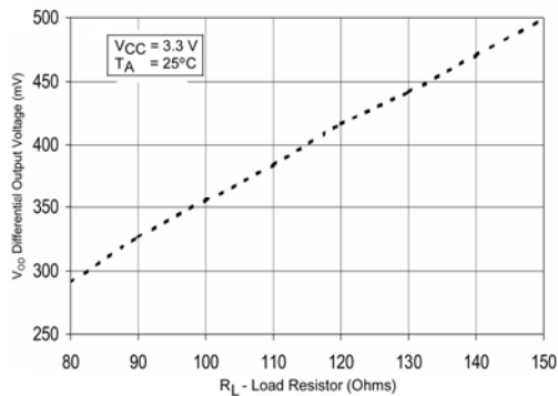
Figure 8. Differential Output Voltage vs. Load Resistor
