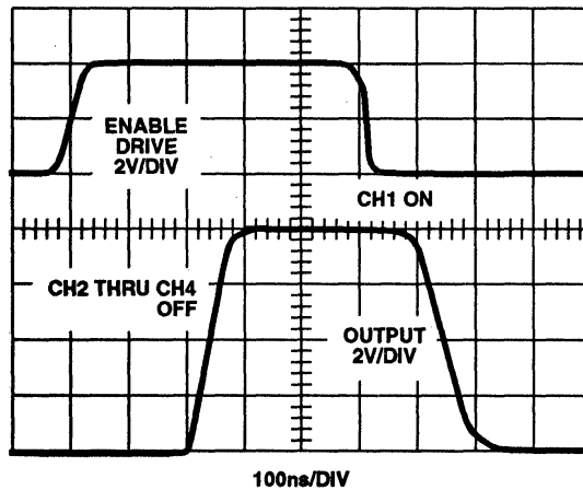
FIGURE 6C. t_{ON(EN)} , t_{OFF(EN)} WAVEFORMS
