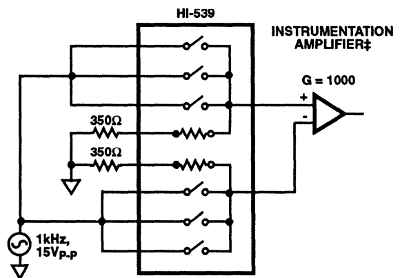
FIGURE 7B. DIFFERENTIAL CROSSTALK TEST CIRCUIT
