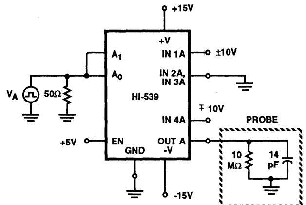
FIGURE 4B. ACCESS TIME TEST CIRCUIT
