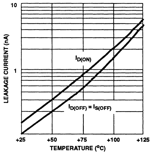
FIGURE 2A. LEAKAGE CURRENT vs TEMPERATURE
