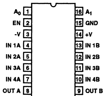
HI1-539 (CDIP) HI3-539 (PDIP) TOP VIEW
