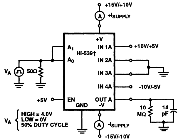
FIGURE 3B. SUPPLY CURRENT TEST CIRCUIT
