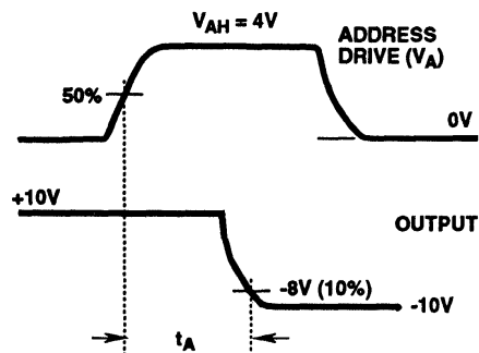
FIGURE 4C. ACCESS TIME MEASUREMENT
