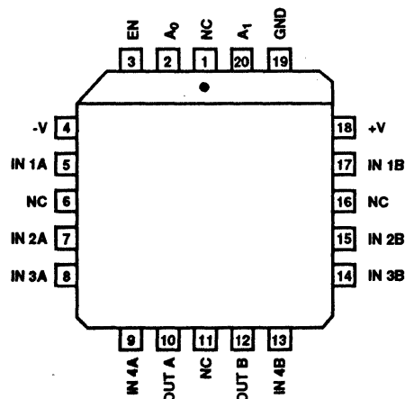
HI4P539 (PLCC) TOP VIEW
