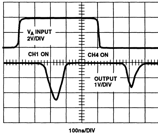
FIGURE 5C. t_{\text{OPEN}} WAVEFORMS
