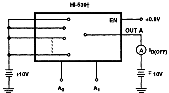
FIGURE 2B. I_{D(OFF)} TEST CIRCUIT (NOTE 1)
