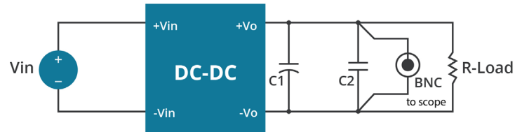
Figure 2 Measuring Output Ripple And Noise
