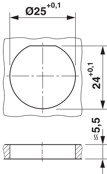
Installation dimensions
