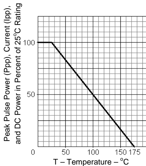
FIGURE 4 DERATING CURVE
