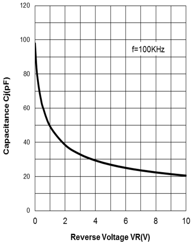
Capacitance vs. Reverse Voltage ( T_a=25^\circ\text{C} )
