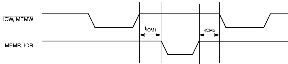
I/O to Memory Command Inactive Time
