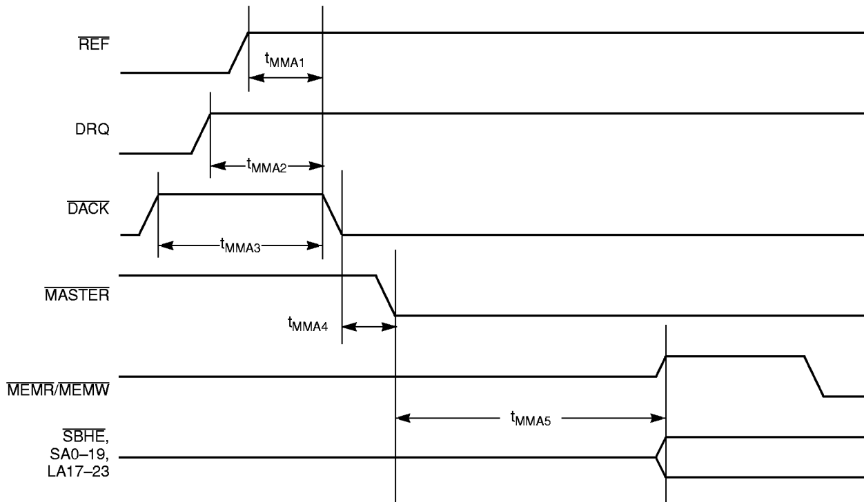
Bus Acquisition
