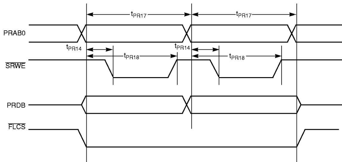
Flash Write on Private Bus
