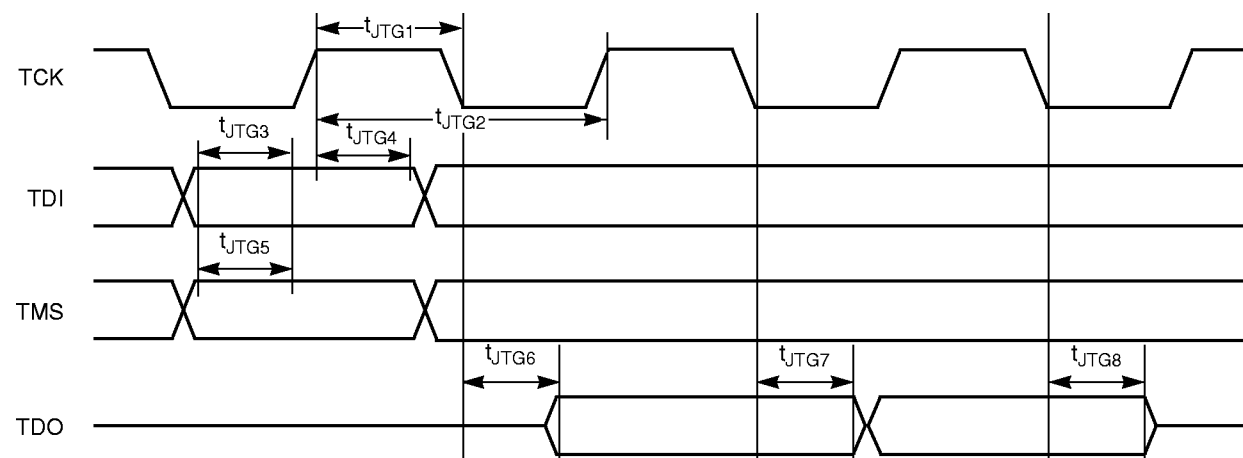
Test Access Port Timing
