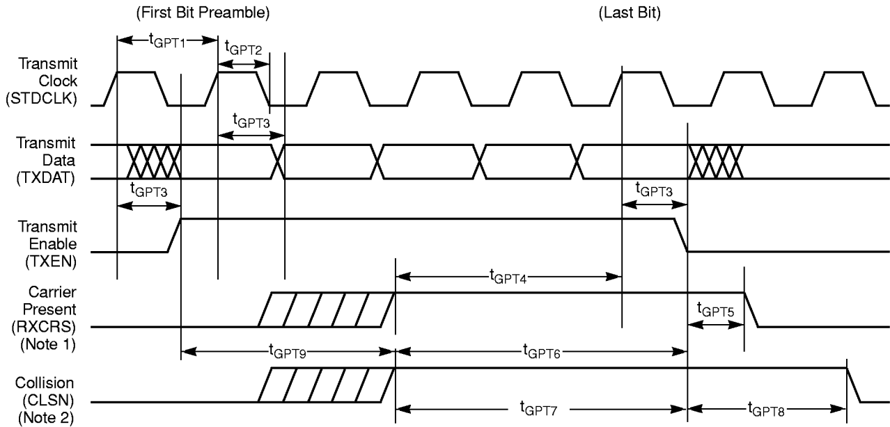
Transmit Timing
