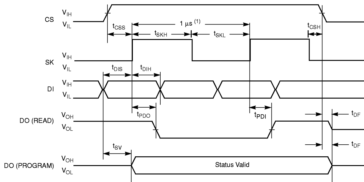
Typical XXC56 Series Serial EEPROM Control Timing
