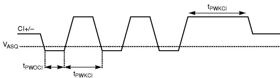
Collision Timing Diagram
