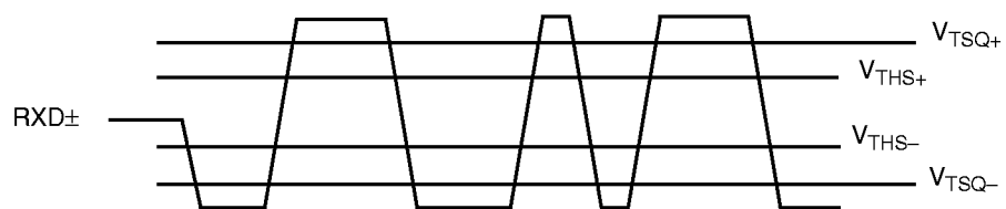
Receive Thresholds (LRT = 0 in CSR15 bit 9)
