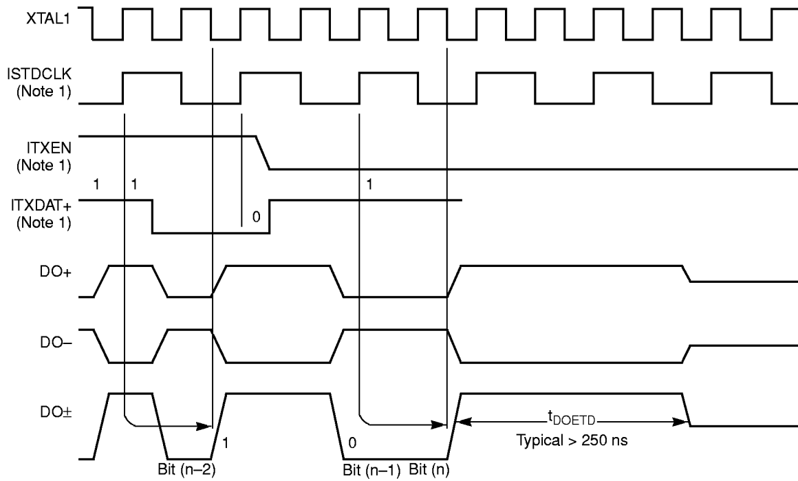
Transmit Timing—End of Packet (Last Bit = 1)
