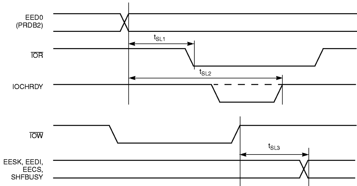
Slave Serial EEPROM Latency Timing
