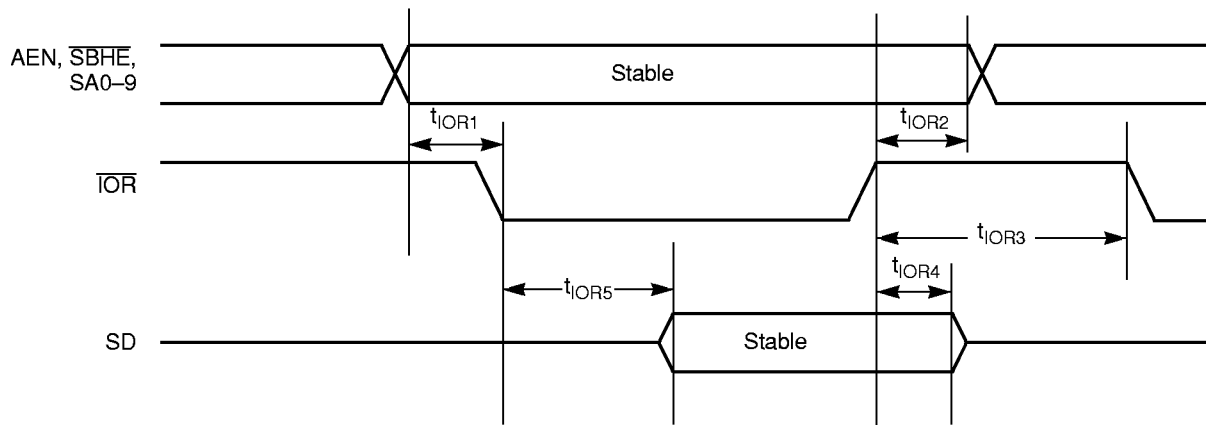
I/O Read without Wait States
