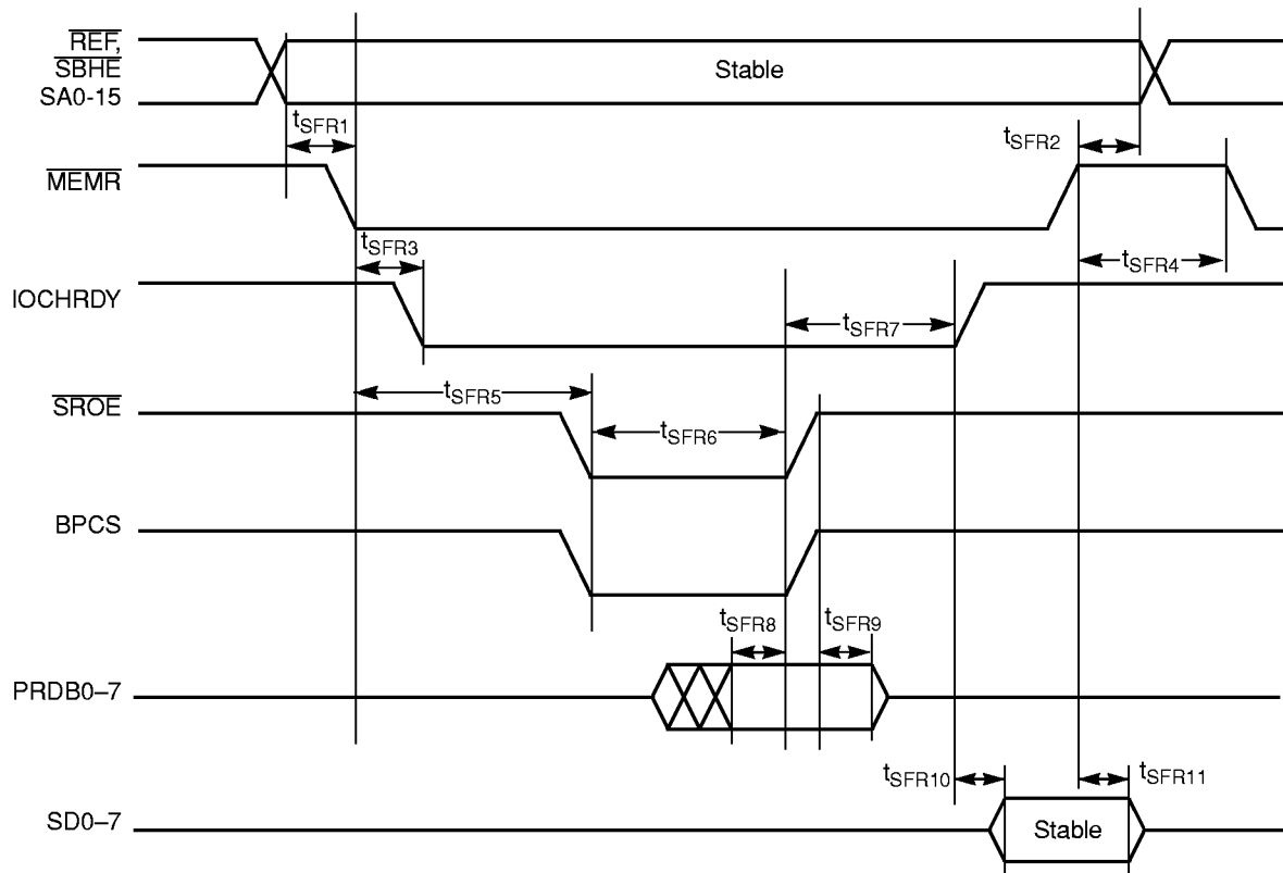
Flash Read Cycle
