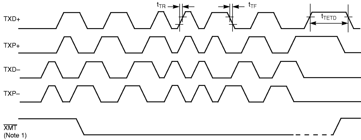
Transmit Timing
