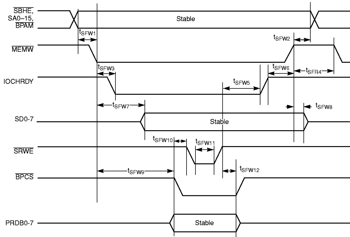
Flash Write Cycle
