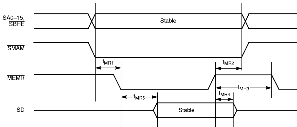
Memory Read without Wait States
