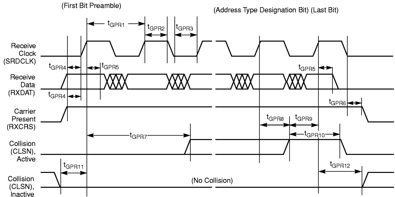
Receive Timing
