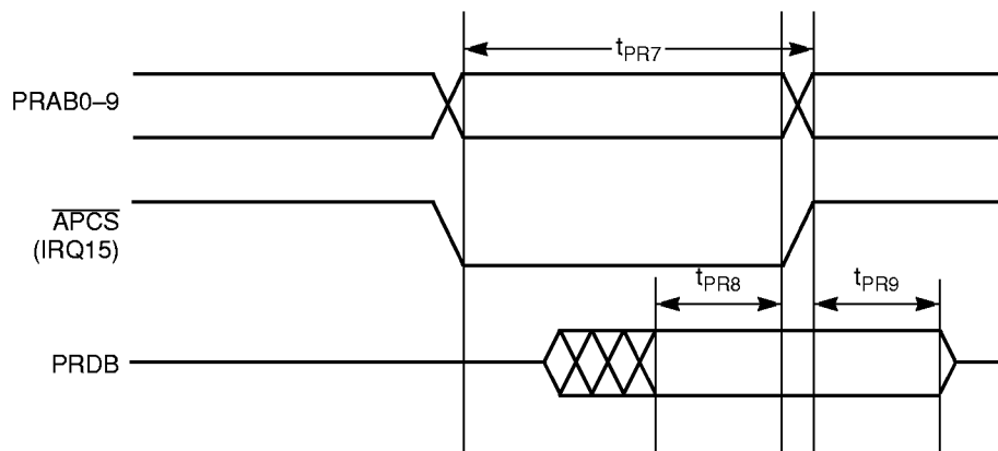
Address PROM Read on Private Bus
