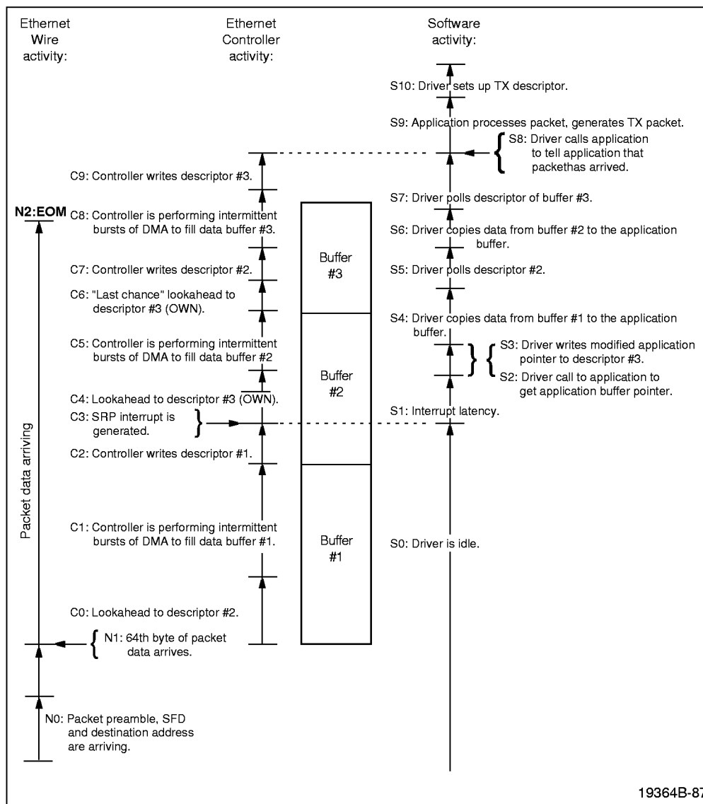
Figure 1. Look Ahead Packet Processing (LAPP) Timeline
