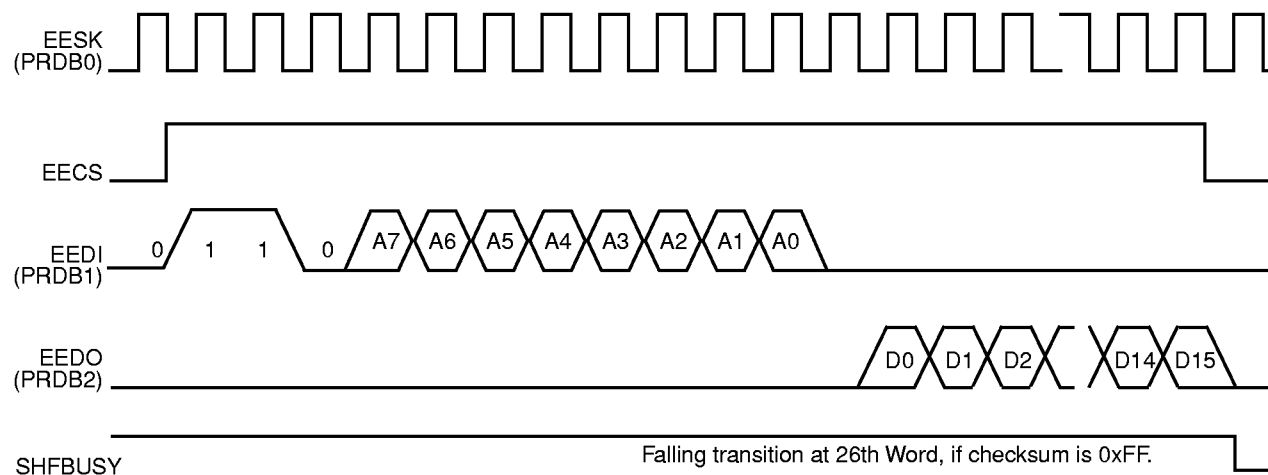
Serial Shift EEPROM Interface Read Timing
