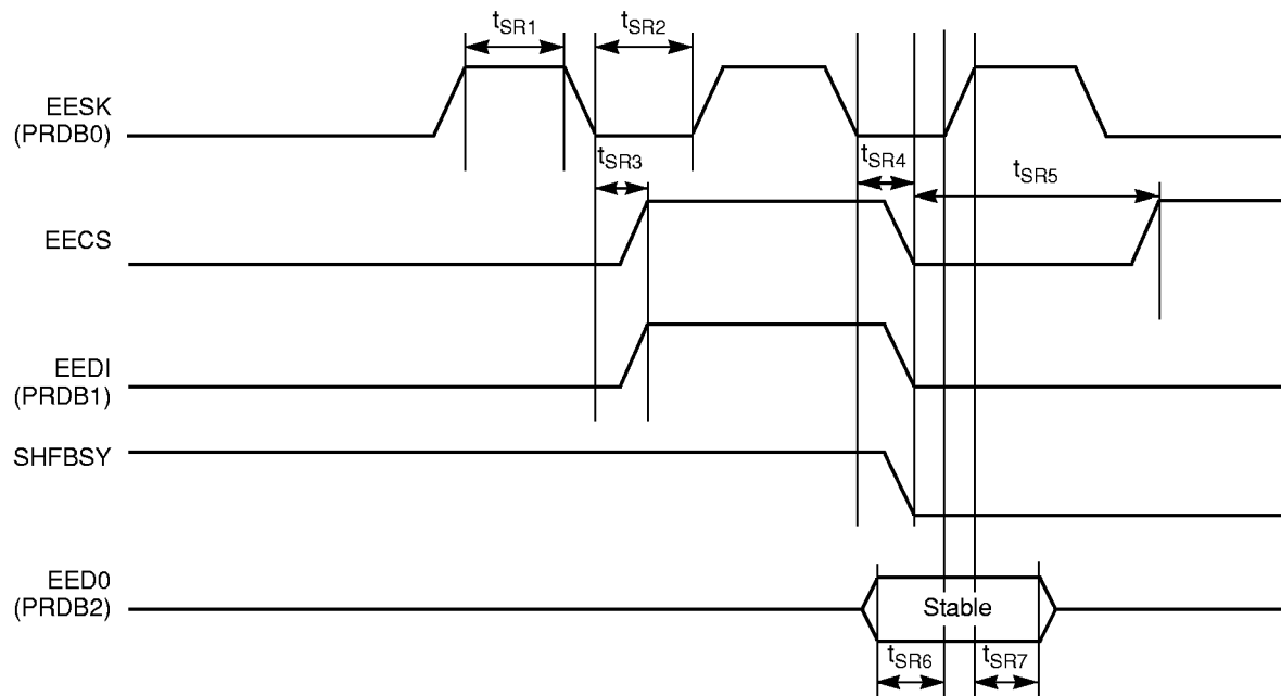
Serial EEPROM Control Timing
