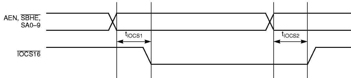
\overline{\text{IOCS16}} Timings
