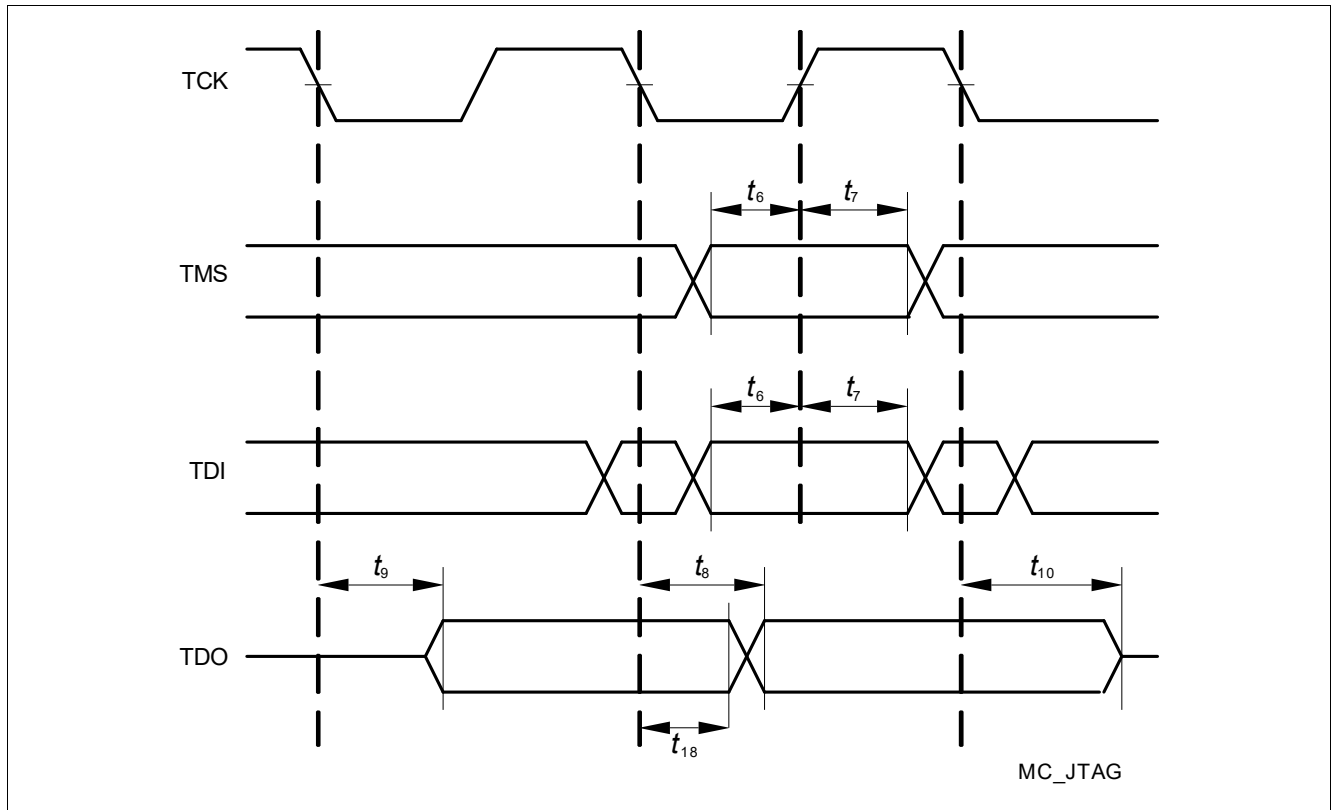
Figure 3-11 JTAG Timing
