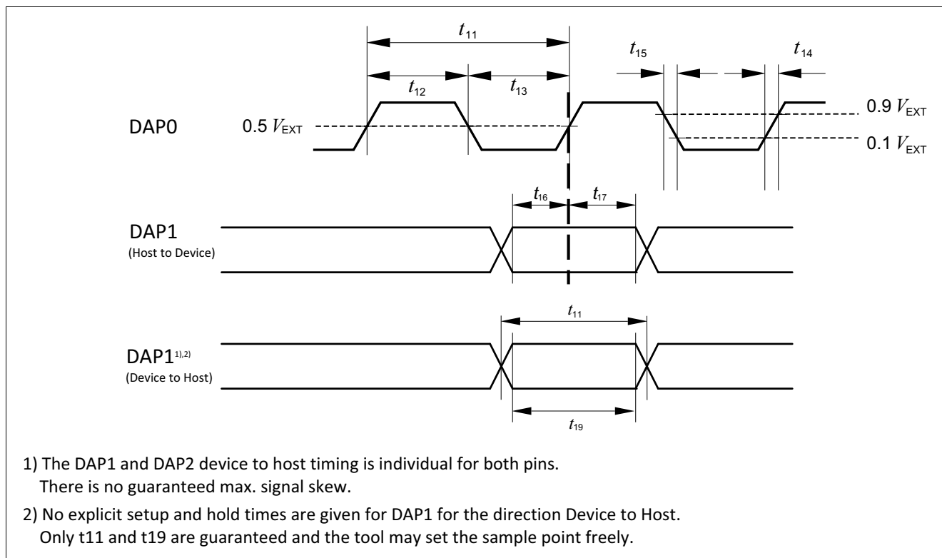
Figure 3-12 DAP Timing
