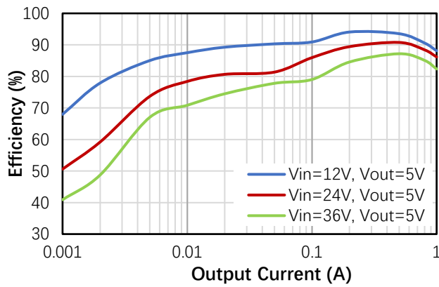
Figure 1. Efficiency Curve
