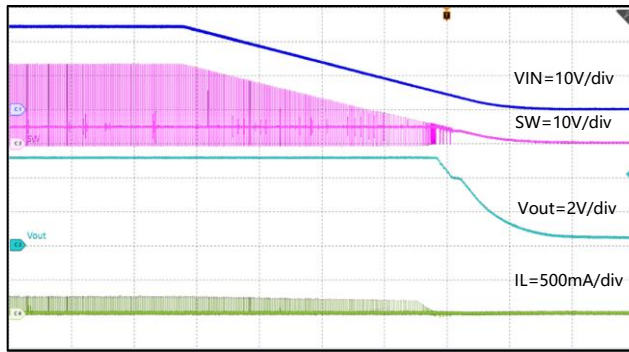
Figure 20. Shut-Down with VIN falling, I_{OUT}=1mA
