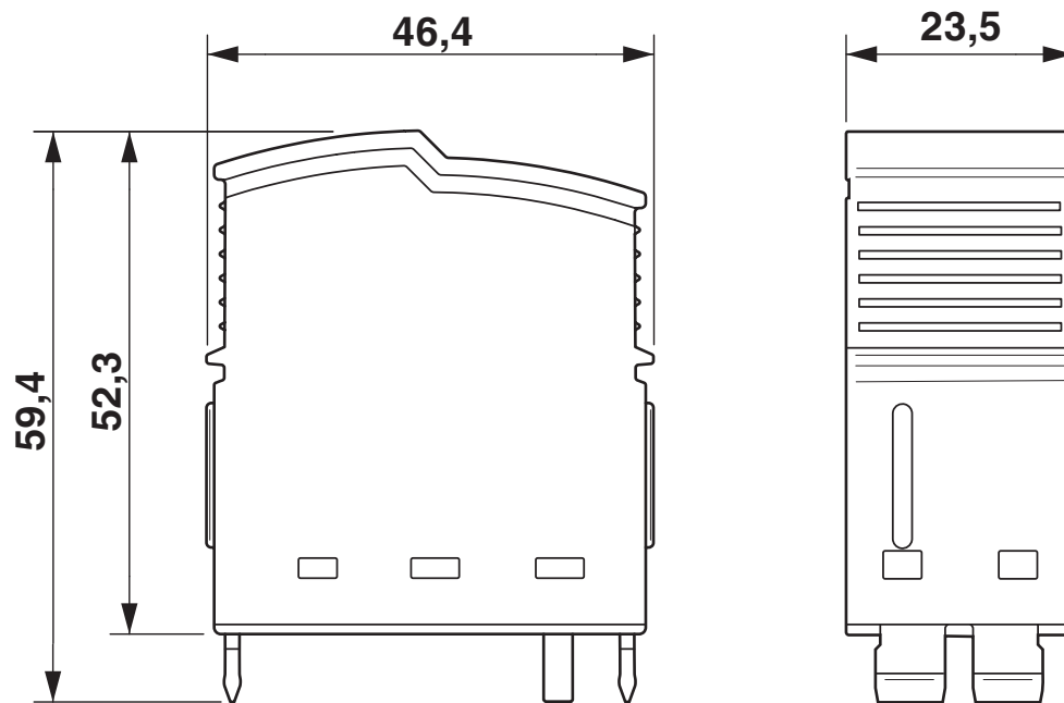
Dimensional drawing
