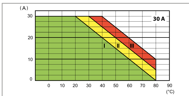
L77-7 Output RMS current v ambient temperature 77.31.x.xxx.80xx
