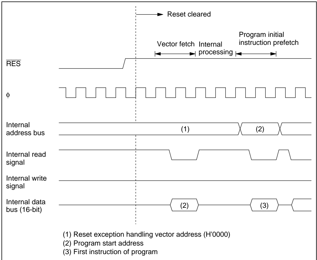
Figure 3.1 Reset Sequence
