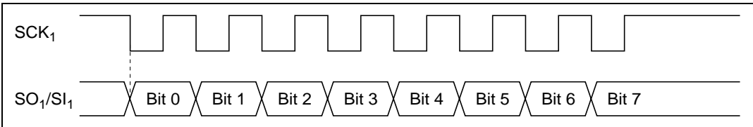
Figure 10.2 Transfer Format
