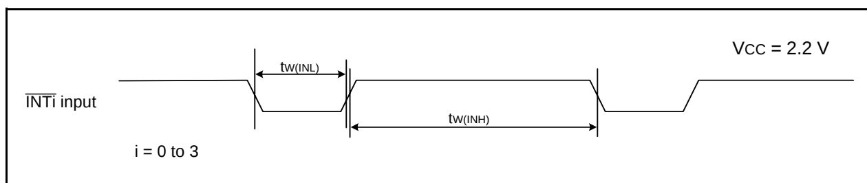
Figure 5.19 External Interrupt INTi Input Timing Diagram when Vcc = 2.2 V
