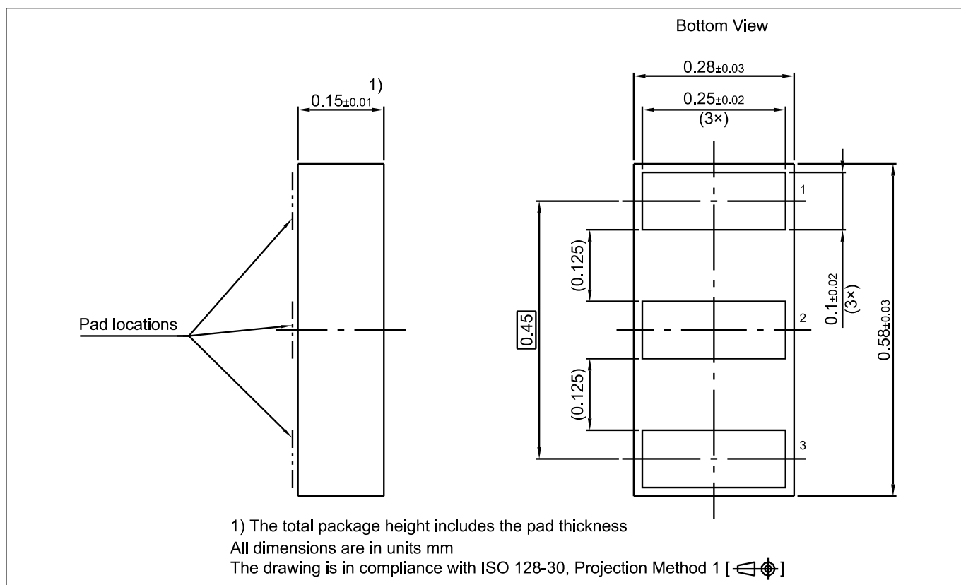
Figure 12 WLL-3-1 package
