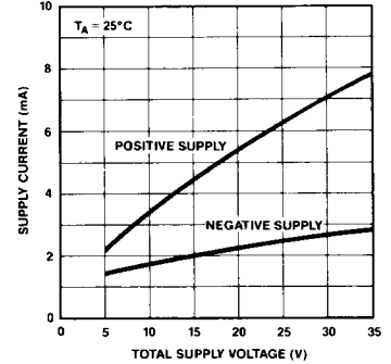
SUPPLY CURRENTS vs SUPPLY VOLTAGE
