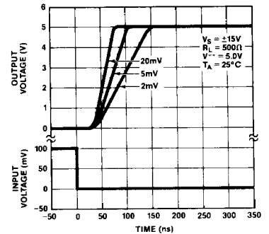
RESPONSE TIMES FOR VARIOUS INPUT OVERDRIVES
