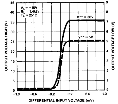
TRANSFER FUNCTION
