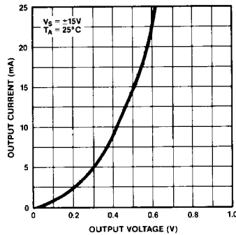
OUTPUT SATURATION VOLTAGE vs OUTPUT CURRENT
