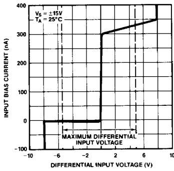
INPUT CHARACTERISTICS
