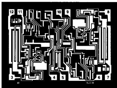
DIE SIZE 0.079 × 0.059 inch, 4661 sq. mils (1.98 × 1.48 mm, 2.93 sq. mm)
