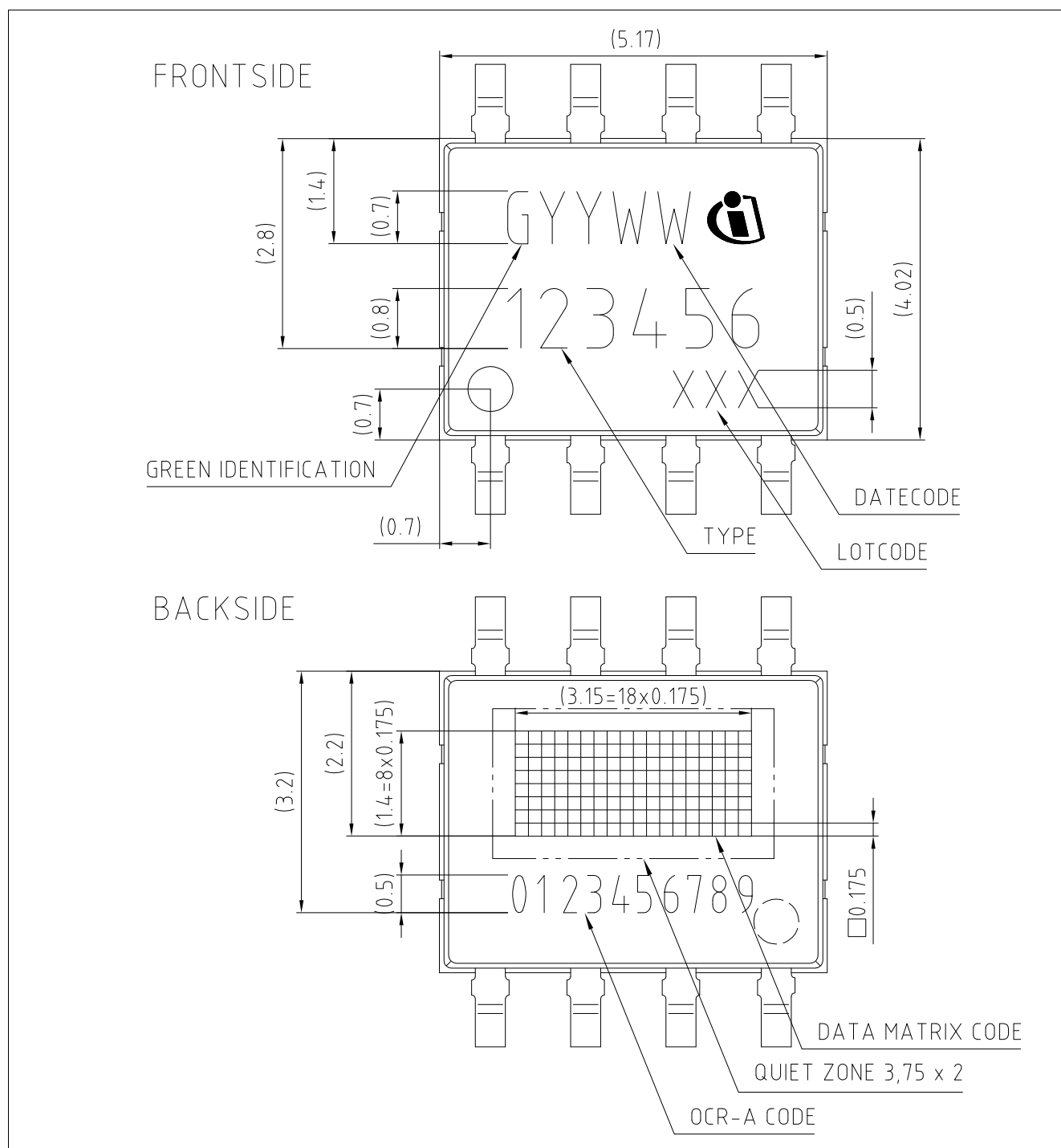
Figure 12 PG-TDSO (Plastic Green Thin Dual Small Outline), package marking
