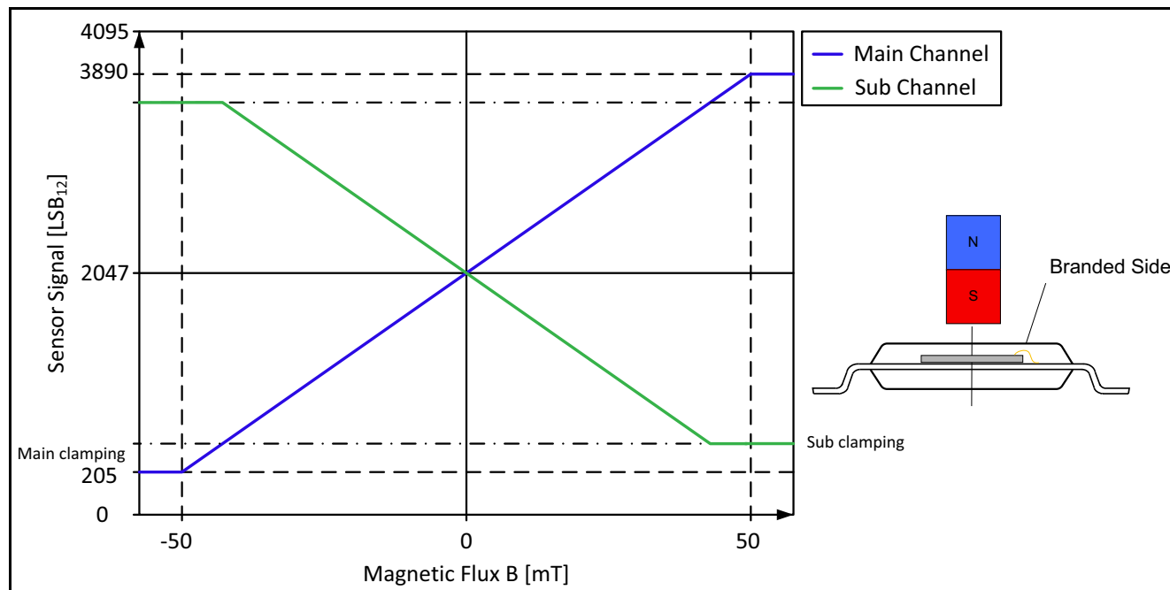
Figure 6 Output characteristic
