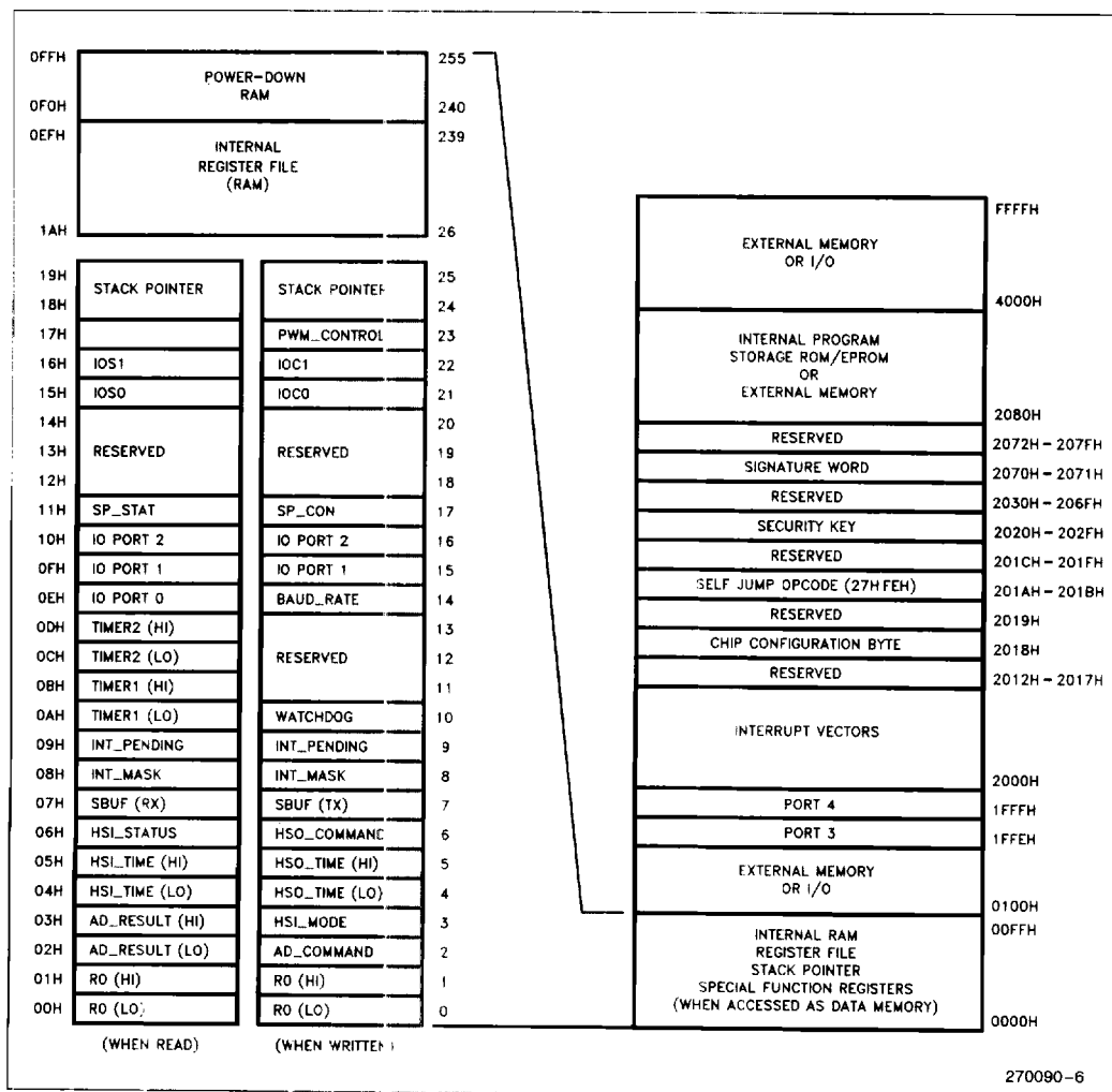
Figure 2. 8X9XBH Memory Map
