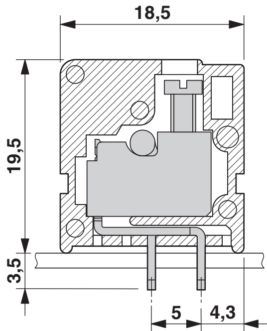
Dimensional drawing
