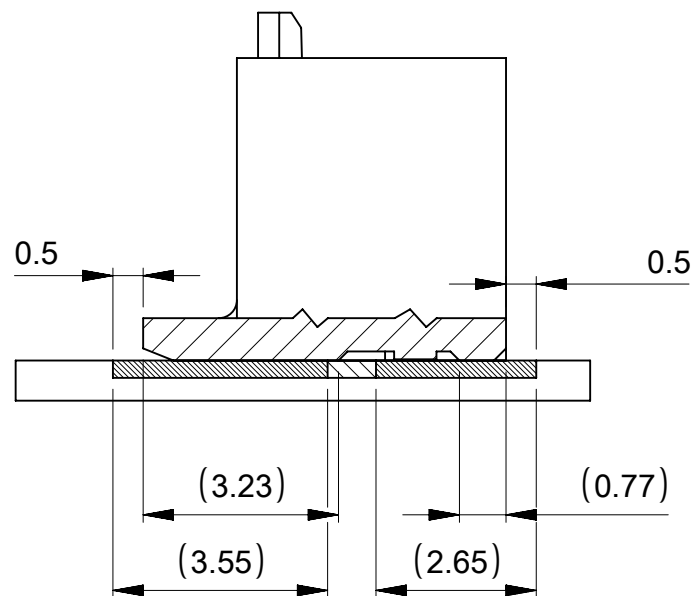
SECTION Z-Z
