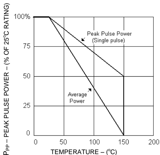
FIGURE 3 Derating Curve
