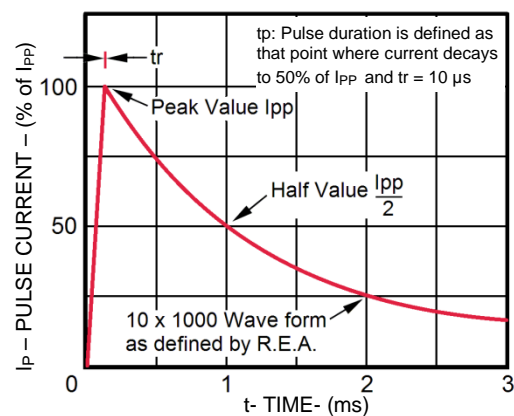
FIGURE 2 Pulse Waveform for 10/1000 \mu s Exponential Surge
