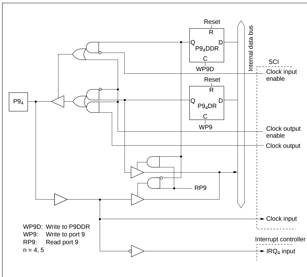
Figure C-8 (c) Port 9 Block Diagram (Pin P9 4 )
