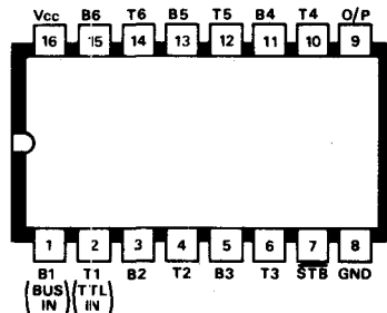
C12 DM8160N 6-bit comparator
