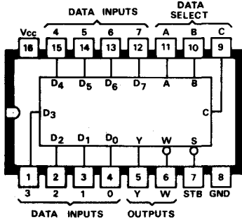
C8 DM8121N 8 channel multiplexer (Tri-state)
