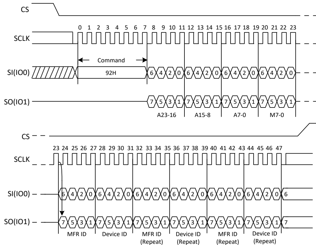
Figure 6. Read Manufacture ID/ Device ID Dual I/O Sequence Diagram
