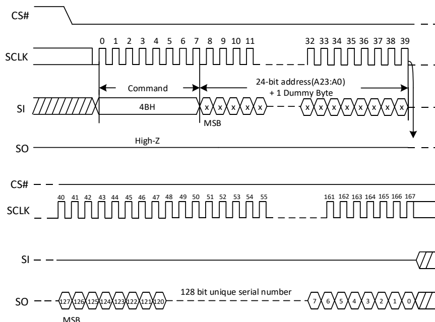
Figure 9. Read Unique ID (RUID) Sequence (Command 4BH)
