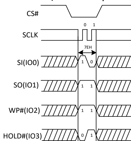
Figure 46a. The Global Block/Sector Lock Sequence Diagram (QPI)
