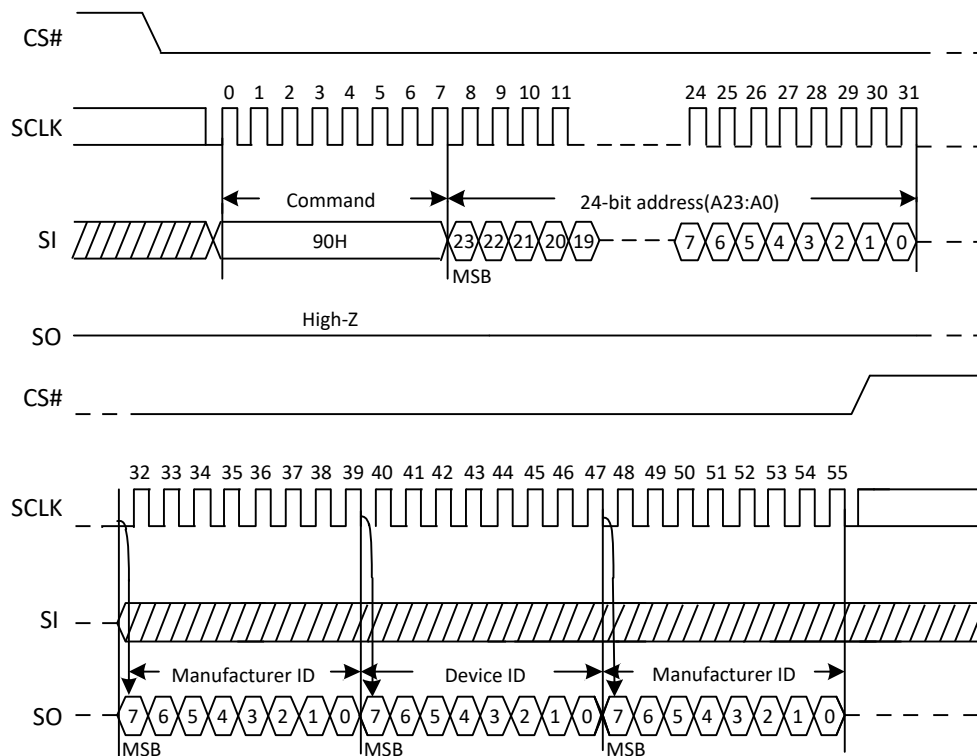
Figure 5. Read Manufacturer ID/ Device ID Sequence Diagram
