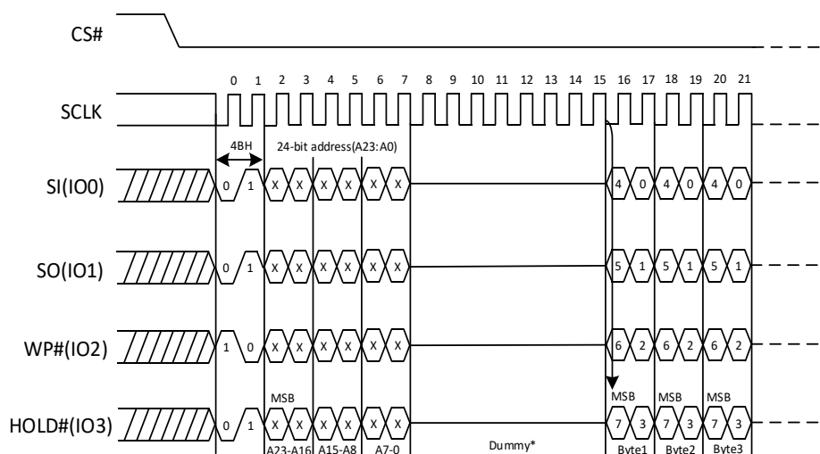
Figure 9a. Read Unique ID (RUID) Sequence (Command 4BH) (QPI)
