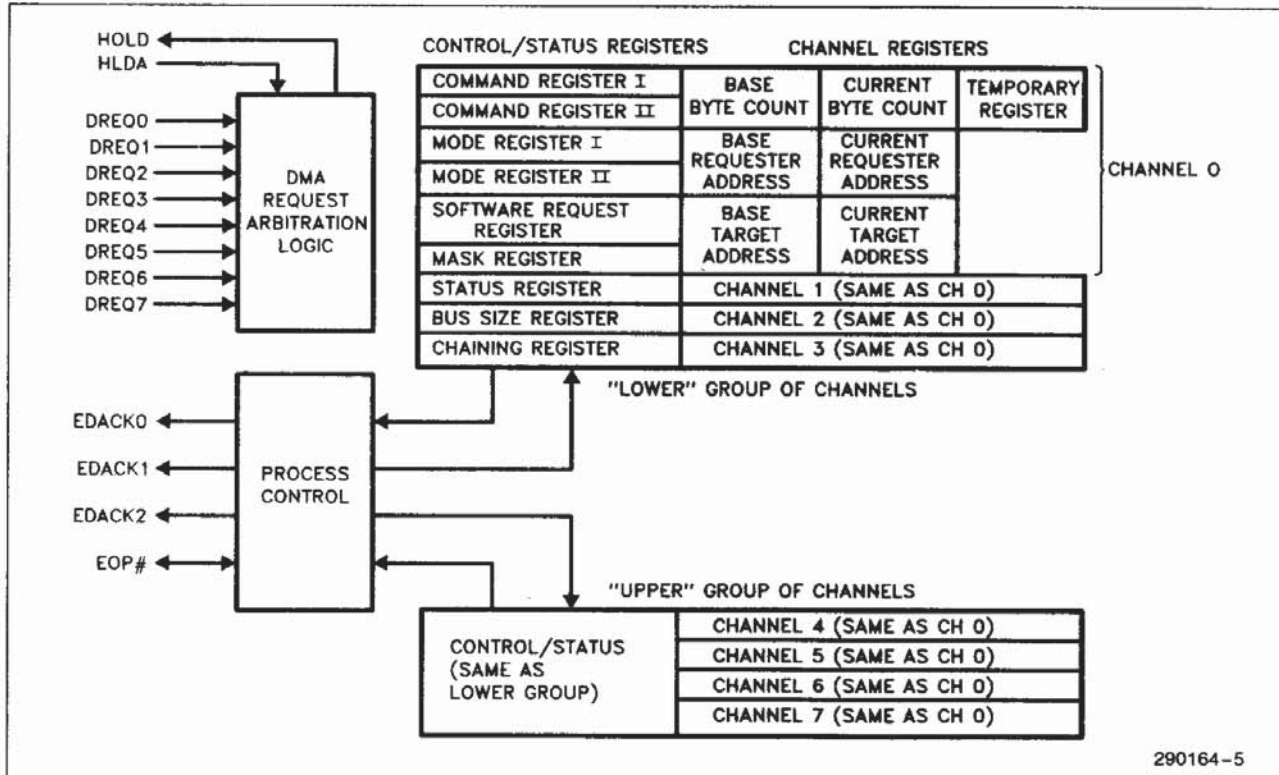
Figure 1-2. 82370 DMA Controller
