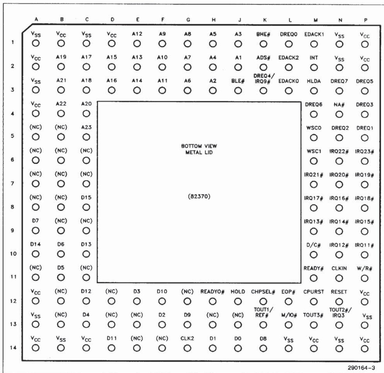
82370 PGA Pinout
