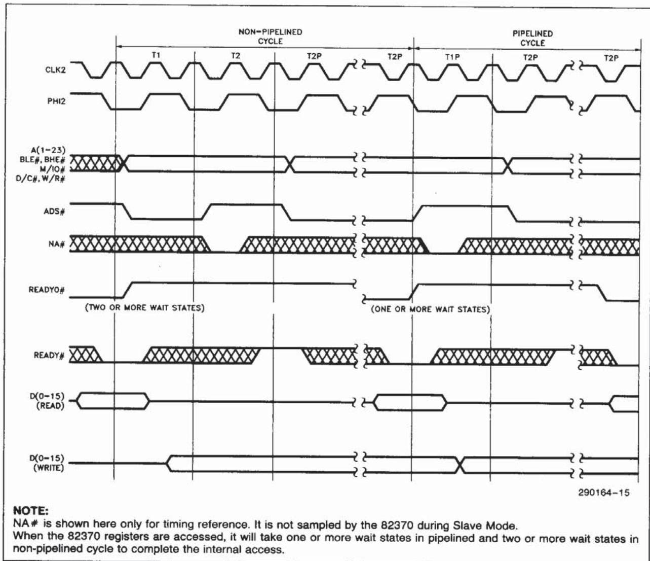
Figure 2-8. Slave Read/Write Timing
