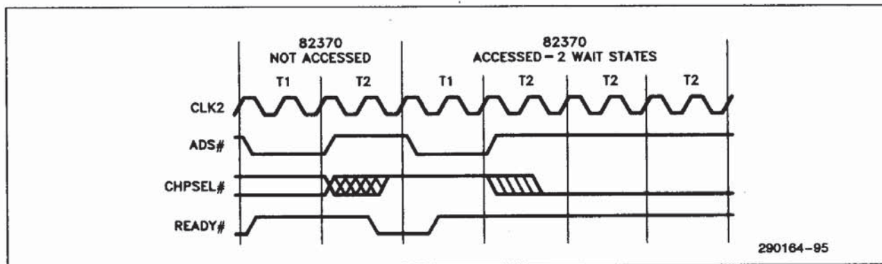
Figure 8-2. CHPSEL# Timing
