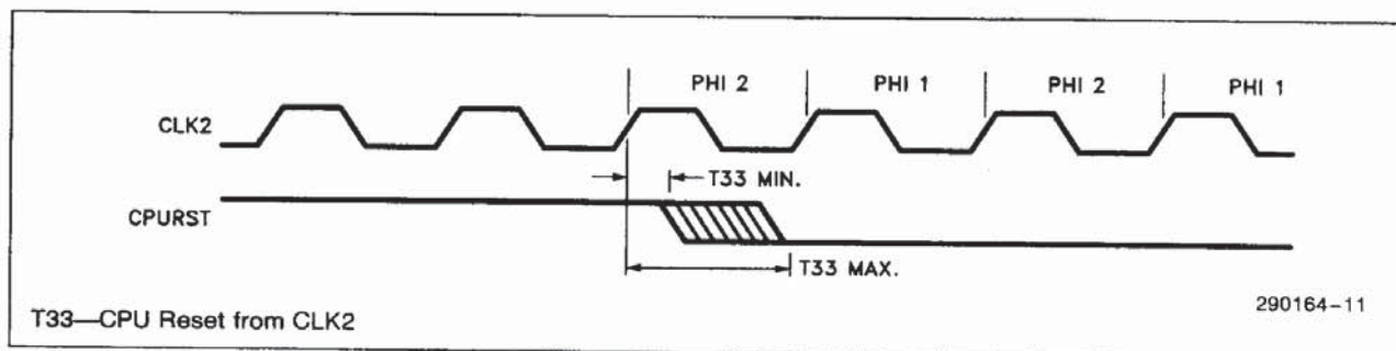
Figure 2-4. CPURST Timing
