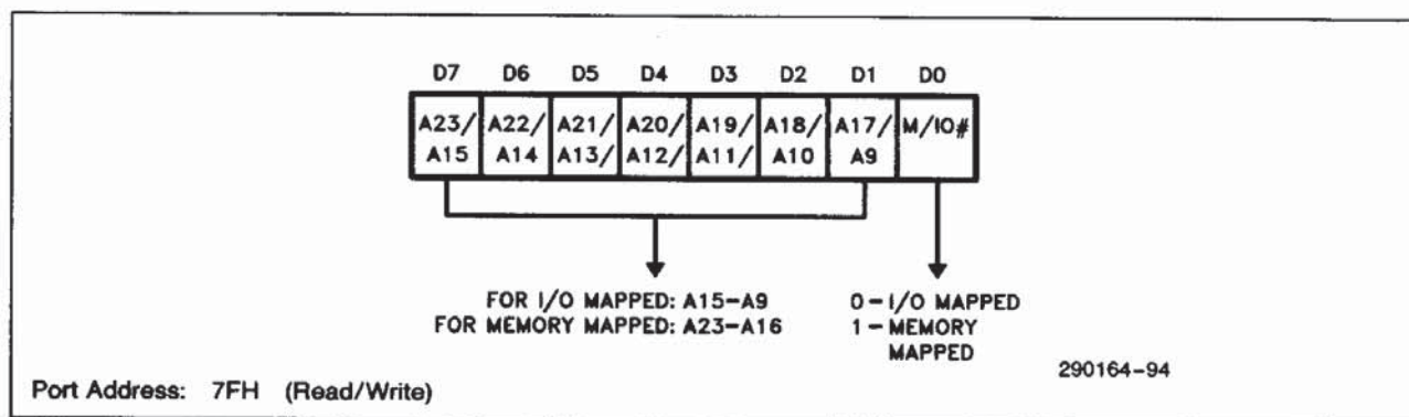
Figure 8-1. Relocation Register
