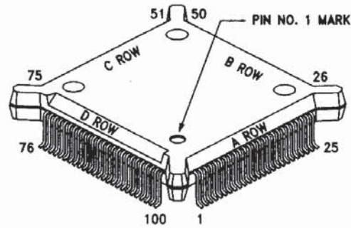
100 Pin Quad Flat-Pack Pin Out (Top View)
