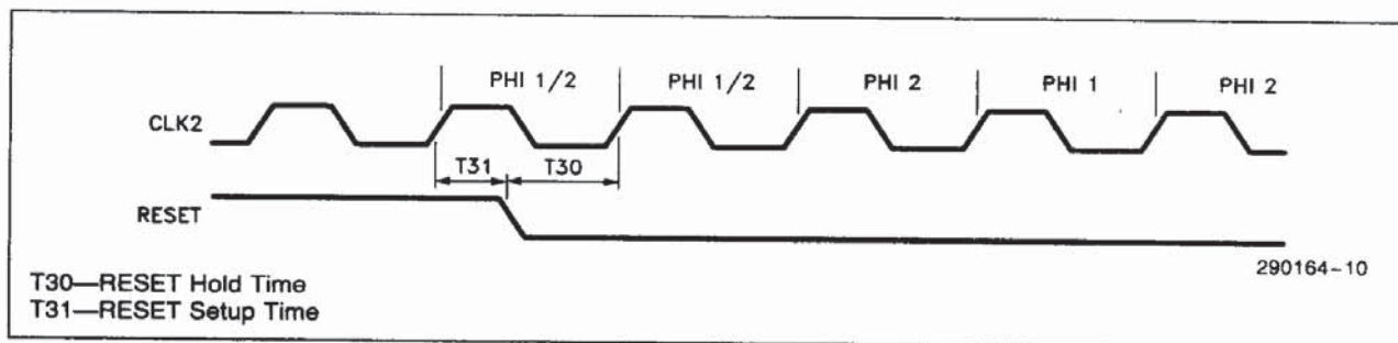
Figure 2-3. RESET Timing
