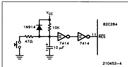
Figure 5. Typical \overline{RES} Timing Circuit
