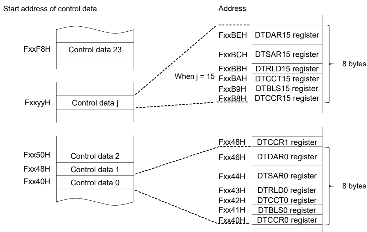
Figure 20 - 3 Control Data Allocation
