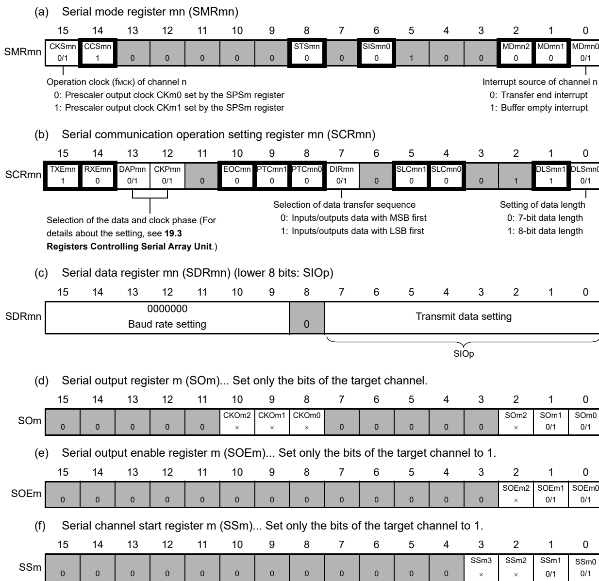
Figure 19 - 50 Example of Contents of Registers for Slave Transmission of Simplified SPI (CSI00, CSI01)
