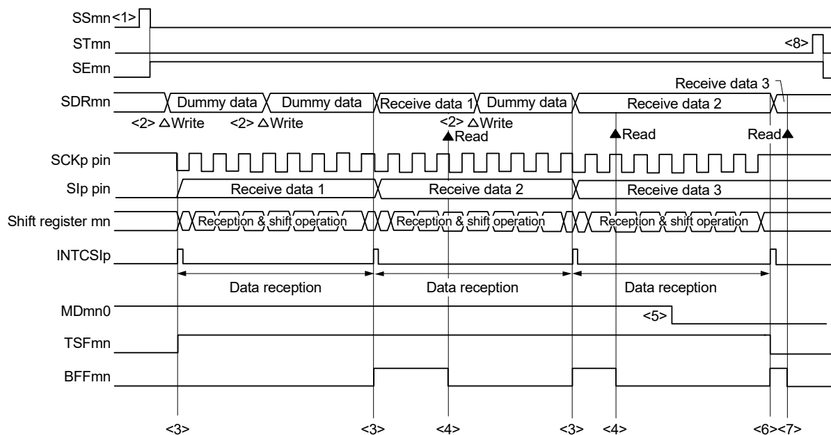
Figure 19 - 40 Timing Chart of Master Reception (in Continuous Reception Mode)
