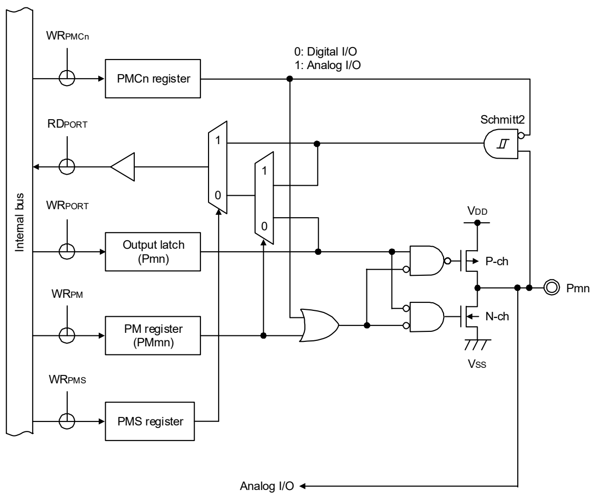
Figure 2 - 3 Pin Block Diagram of Pin Type 6-3-2
