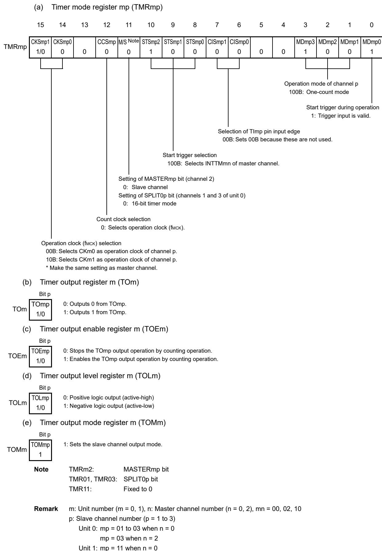
Figure 6 - 78 Example of Set Contents of Registers When PWM Function (Slave Channel) Is Used
