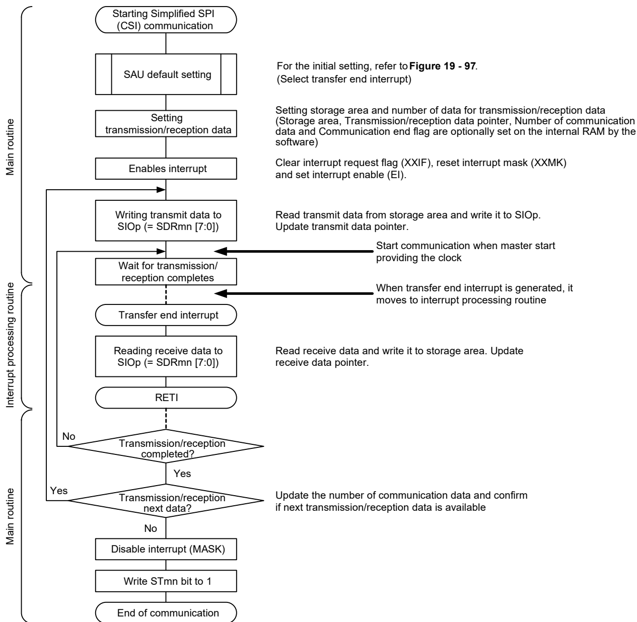
Figure 19 - 101 Flowchart of Slave Transmission/Reception (in Single- Transmission/Reception Mode)
