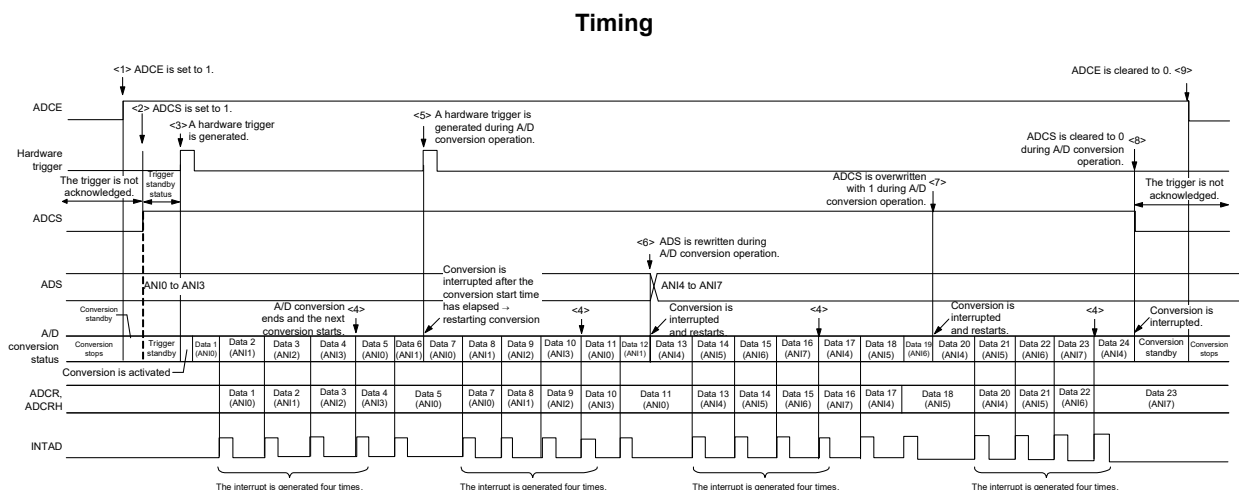
Figure 16 - 25 Example of Hardware Trigger No-Wait Mode (Scan Mode, Sequential Conversion Mode) Operation
