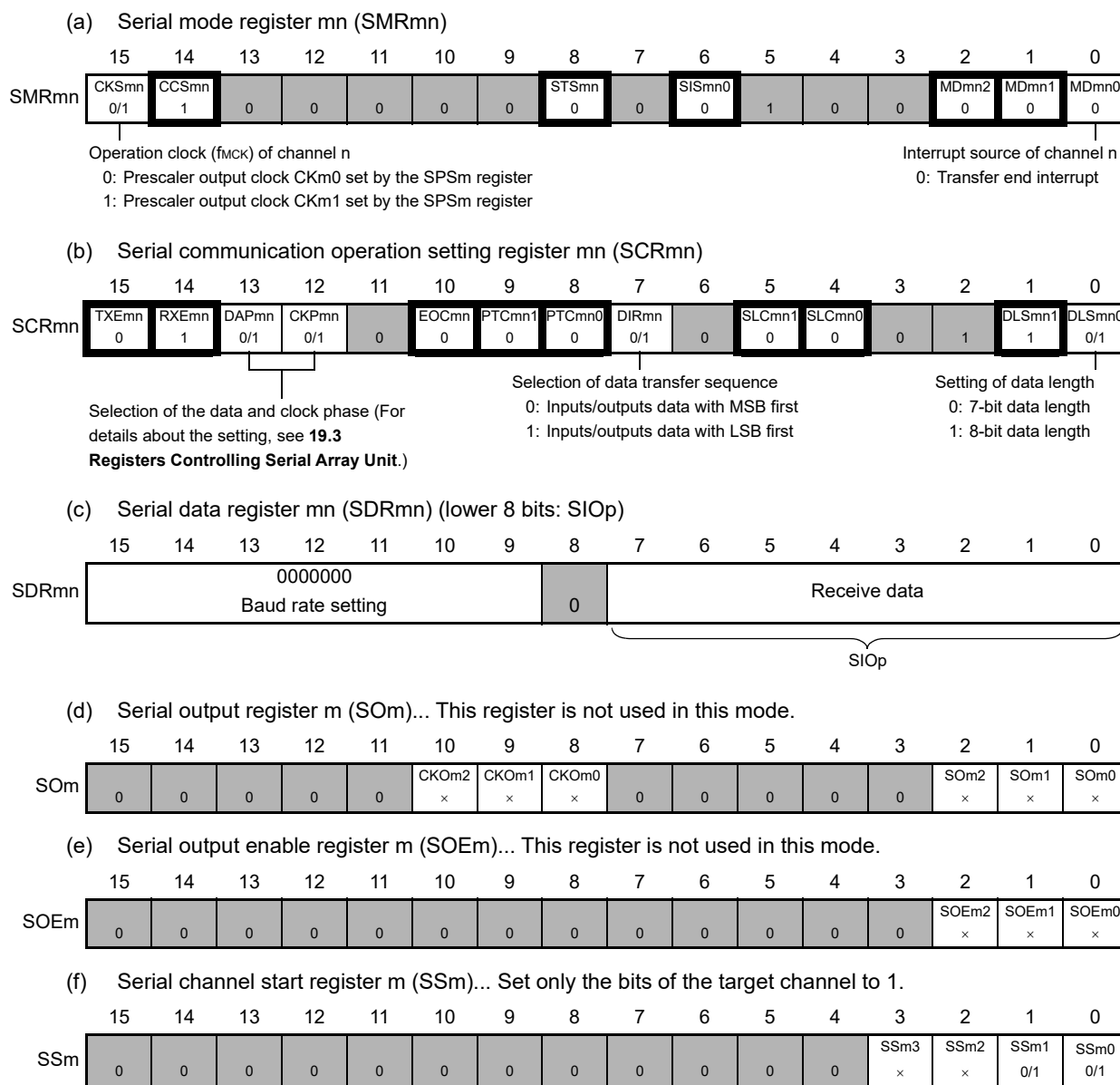
Figure 19 - 58 Example of Contents of Registers for Slave Reception of Simplified SPI (CSI00, CSI01)
