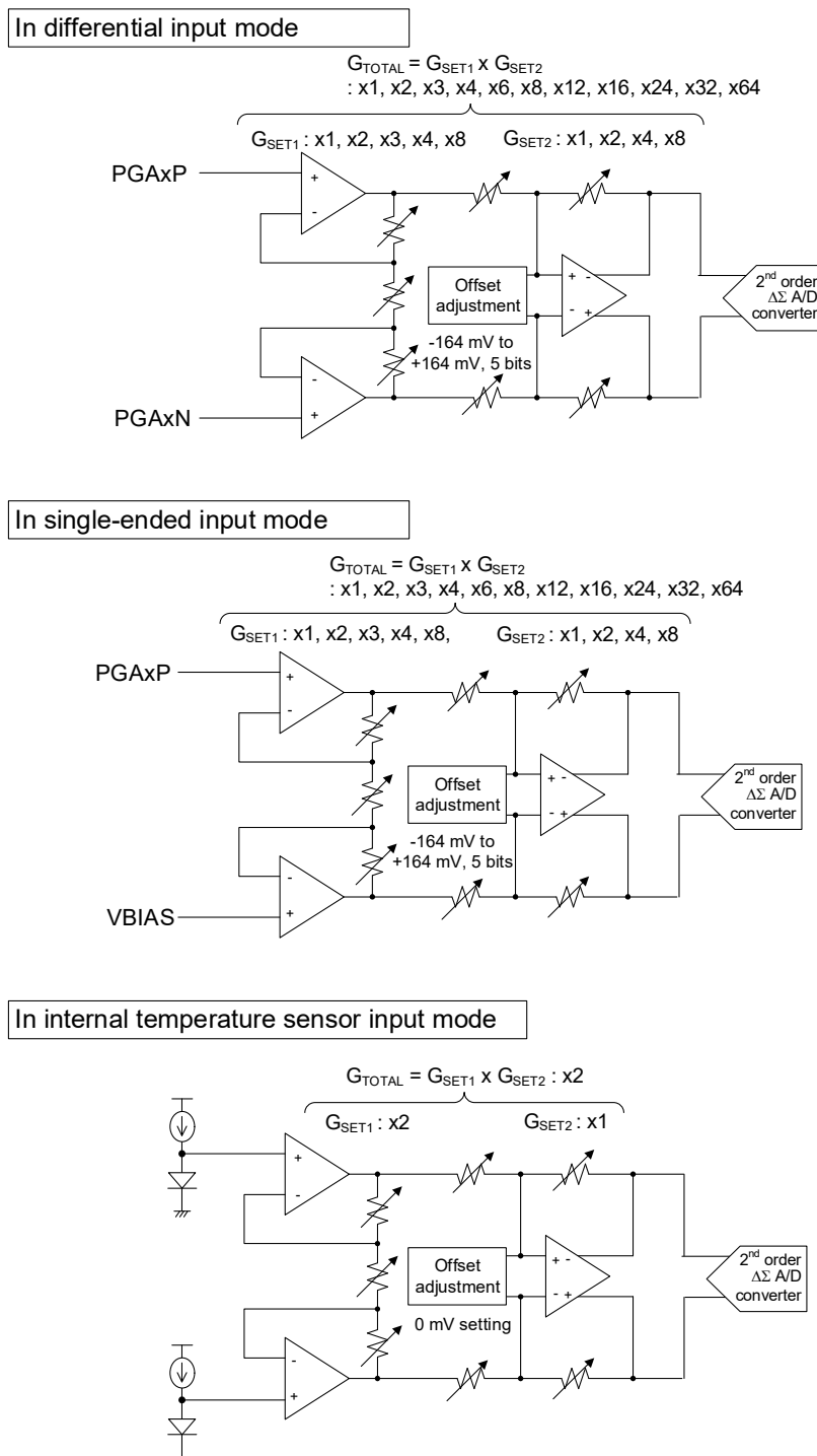
Figure 14 - 4 Block Diagram of Programmable Gain Instrumentation Amplifier (PGA)
