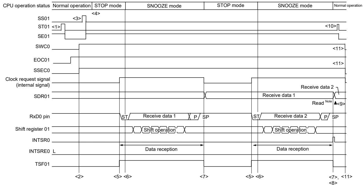
Figure 19 - 124 Timing Chart of SNOOZE Mode Operation (EOCm1 = 1, SSECm = 1)
