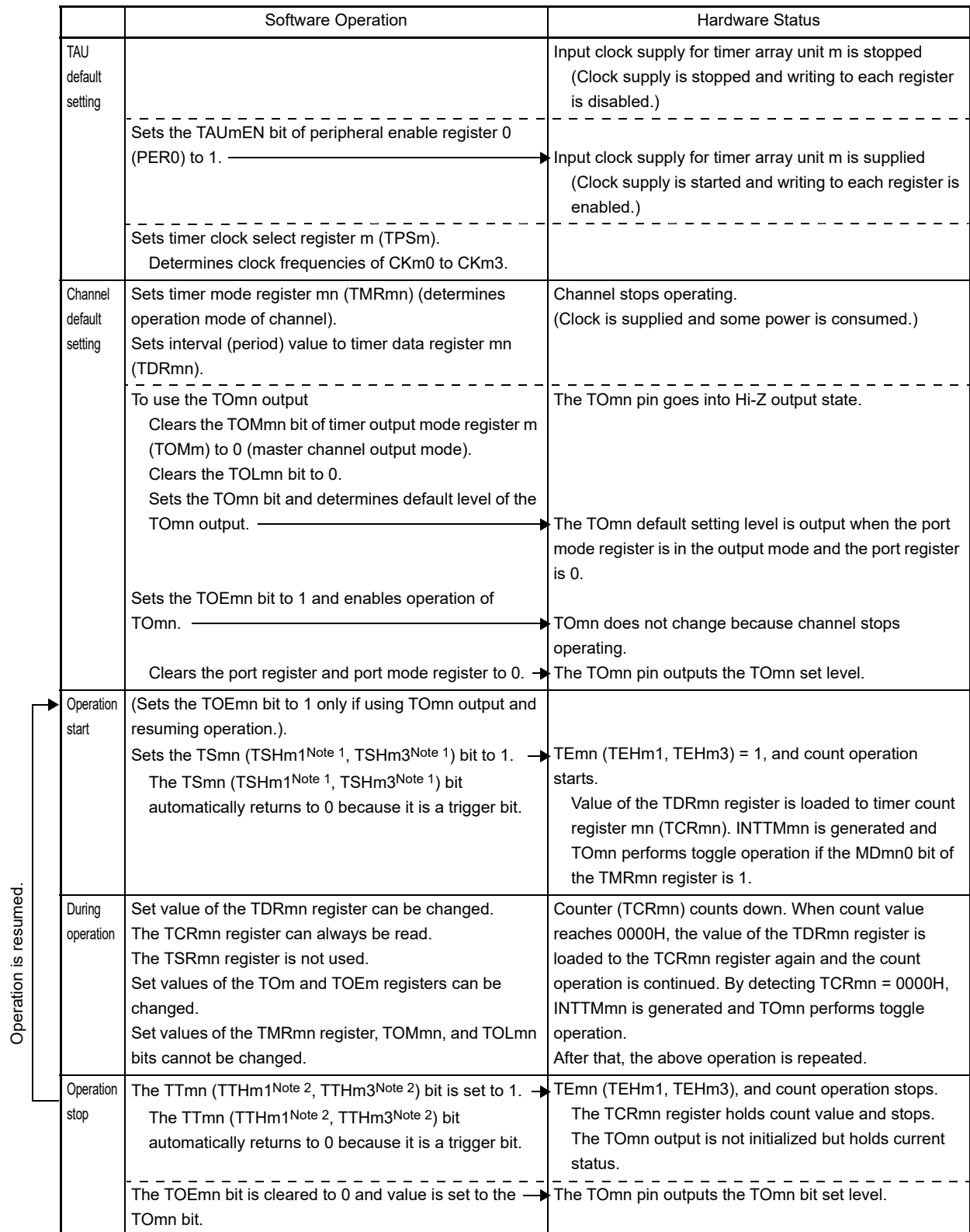
Figure 6 - 51 Operation Procedure of Interval Timer/Square Wave Output Function (1/2)
