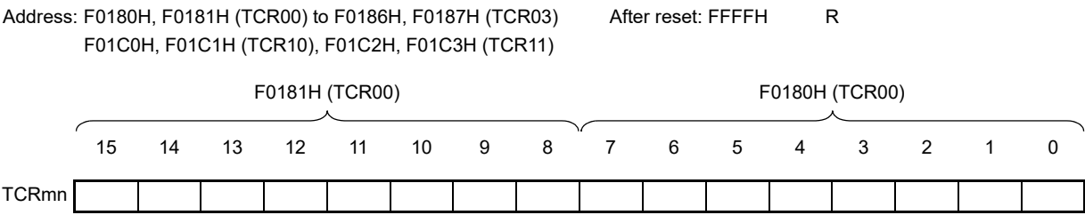
Figure 6 - 9 Format of Timer counter register mn (TCRmn)
