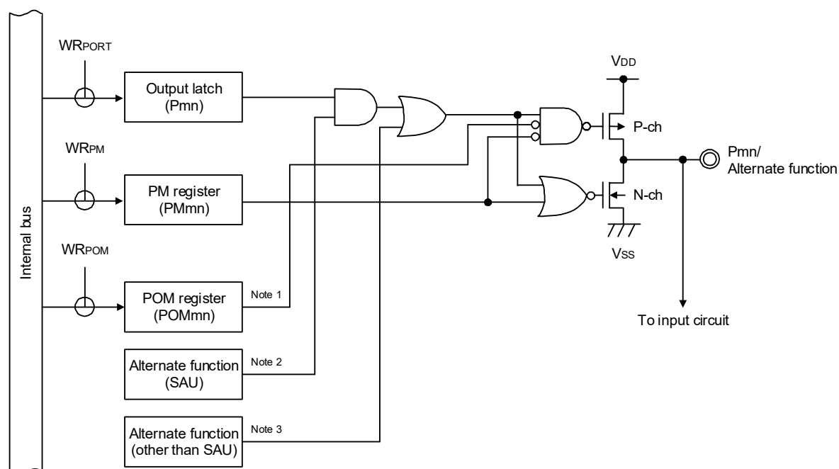
Figure 4 - 7 Basic Configuration of Output Circuit for Pins
