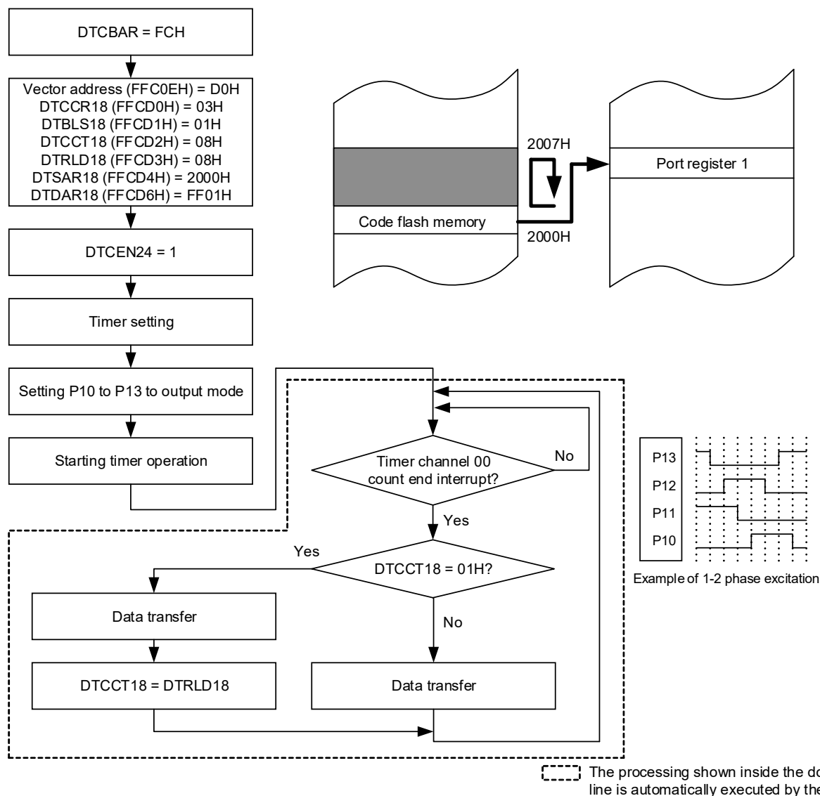
Figure 20 - 19 Example of using repeat mode - 1: Outputting a stepping motor control pulse using ports
