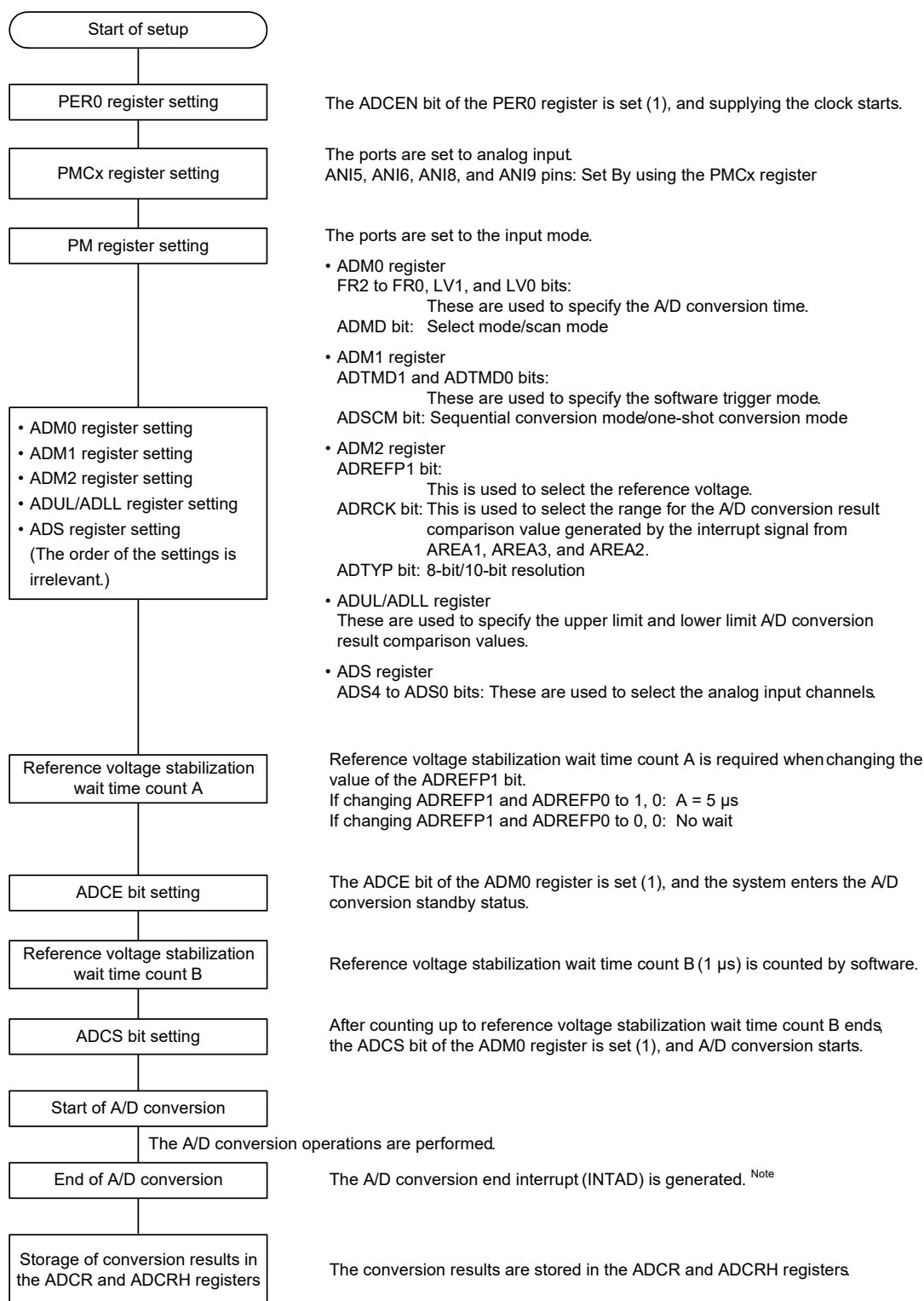
Figure 16 - 31 Setting up Software Trigger Mode
