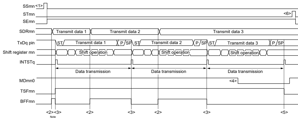
Figure 19 - 112 Timing Chart of UART Transmission (in Continuous Transmission Mode)
