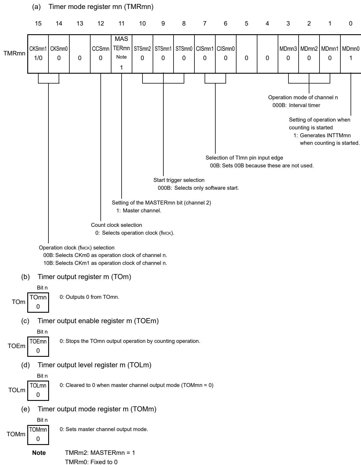
Figure 6 - 77 Example of Set Contents of Registers When PWM Function (Master Channel) Is Used
