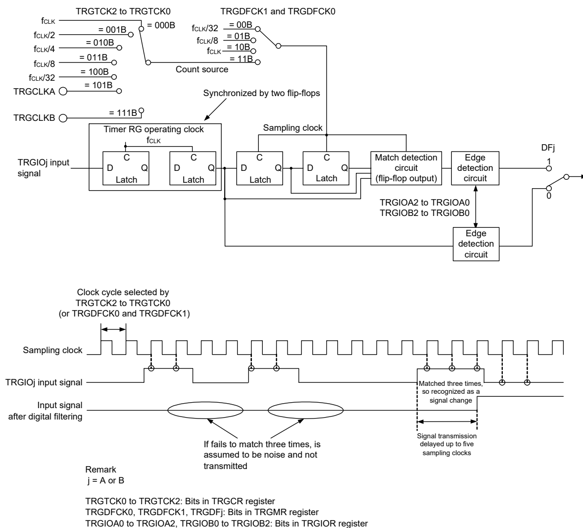
Figure 8 - 15 Block Diagram of Digital Filter
