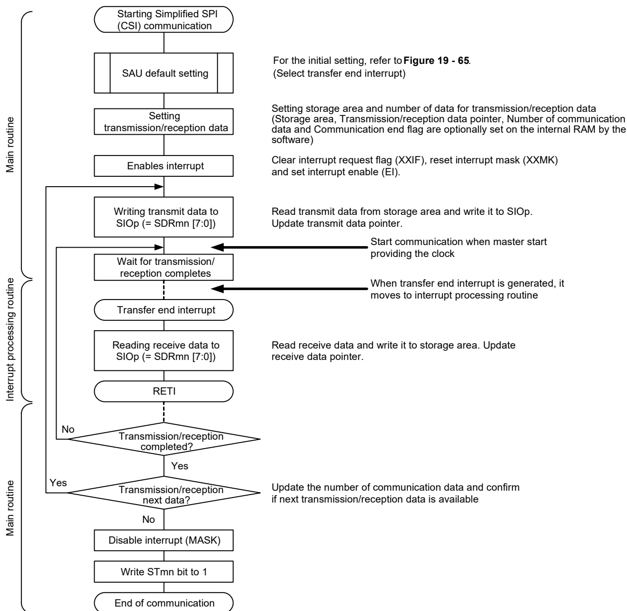
Figure 19 - 69 Flowchart of Slave Transmission/Reception (in Single- Transmission/Reception Mode)
