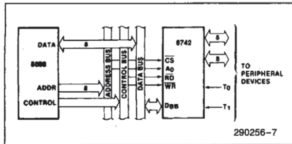
Figure 3. 8088-8742 Interface
