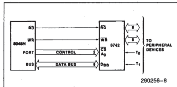
Figure 4. 8048H-8742 Interface
