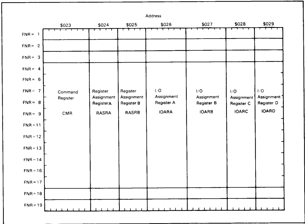
Figure 5. Function Table Configuration
