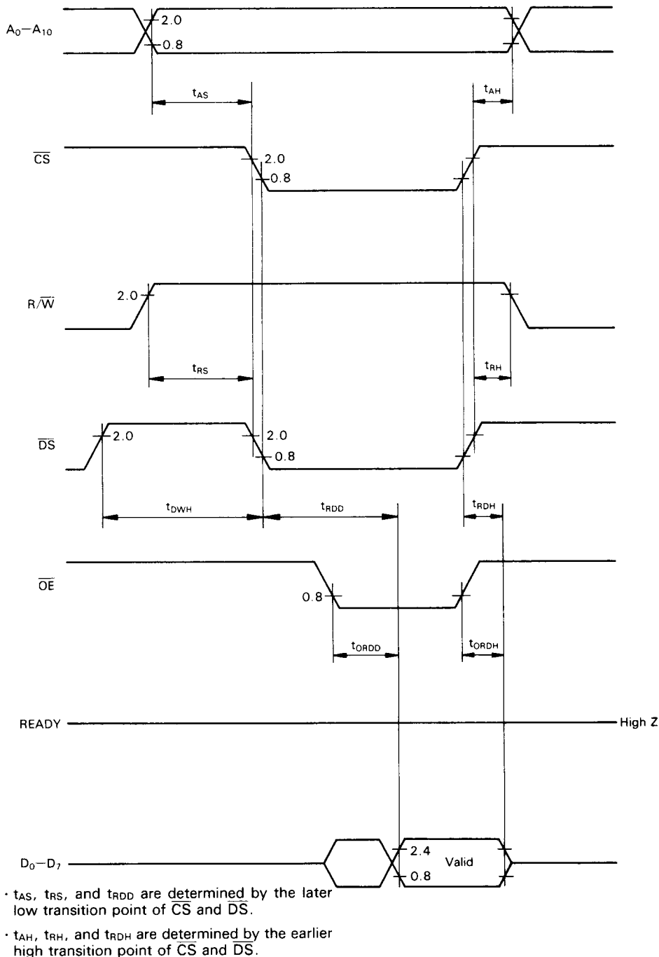
Figure 18. Read Cycle Bus Timing (RAM)
