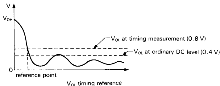
Timing Measurement point of V_{OL}
