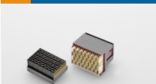
TE Part #2302785-1 RA PLUG ASSY,7ROW,CENTER,VPX, MG RT3
