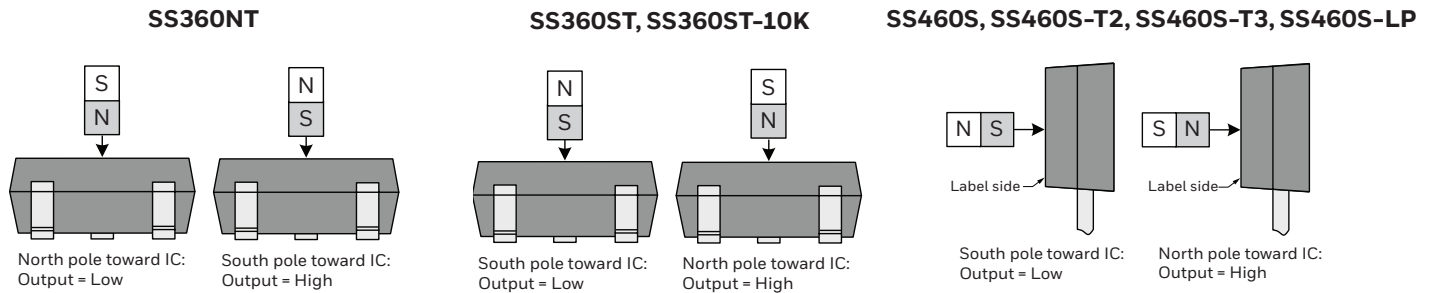
Figure 4. Magnetic Activation
